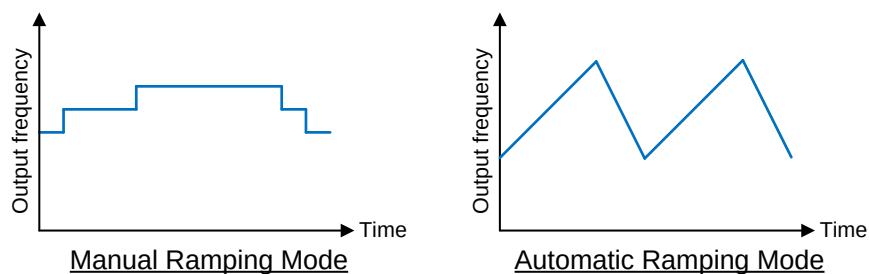
Figure 34. Ramping Modes
