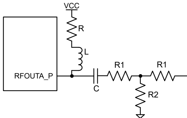
Figure 7-5. Inductor and Resistor Pullup
