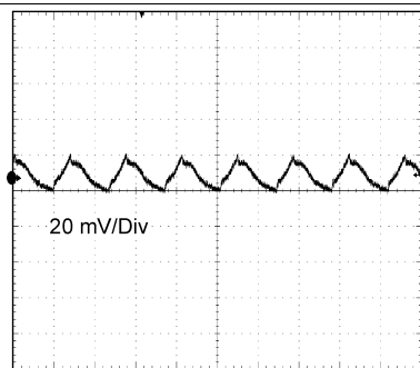
Figure 33. Output Ripple
