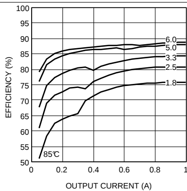
Figure 15. Efficiency 12-V Input at 85°C
