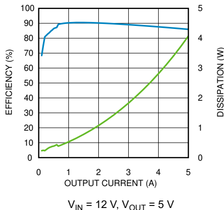
Figure 7-4. Efficiency
