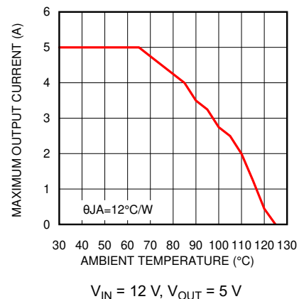
Figure 7-5. Thermal Derating Curve
