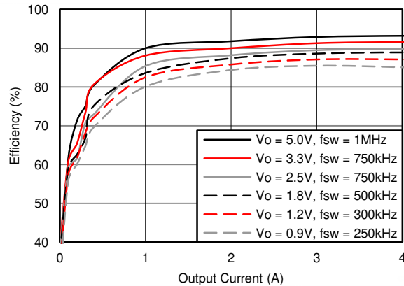
Figure 1. Efficiency versus Output Current
