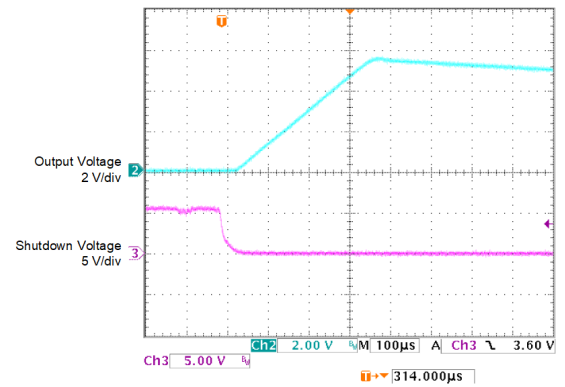
Figure 5-52. Enable Transient Response vs Time ( I_L = 1\text{mA} , C_L = 10\mu\text{F} )
