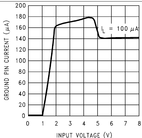
Figure 1. Quiescent Current
