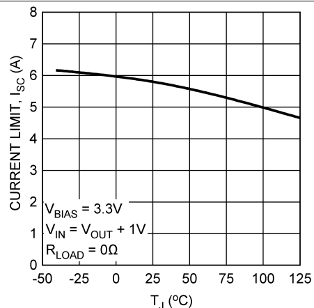
Figure 6. Output Current Limit ( I_{SC} ) vs Temperature
