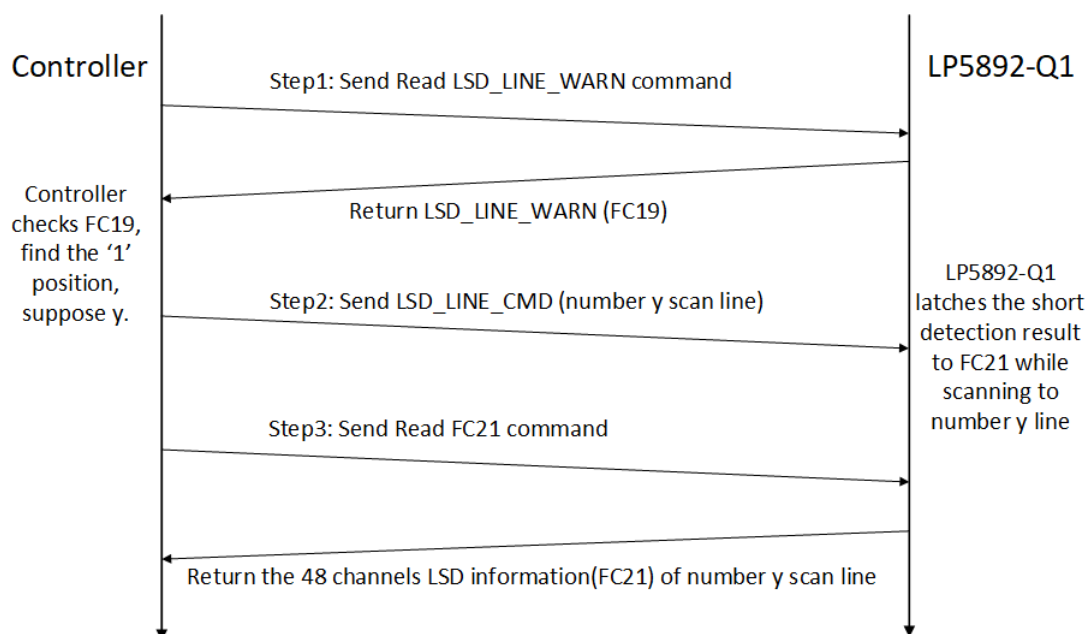
Figure 6-11. Steps to Read LED Short Information
