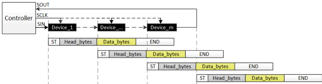
Figure 6-18. Data Write Command with Broadcast
