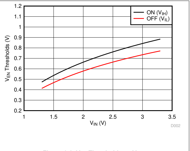
Figure 6-2. V_{EN} Thresholds vs V_{IN}
