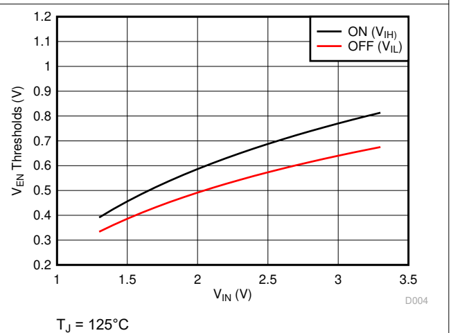
Figure 6-2. V_{EN} Thresholds vs V_{IN}
