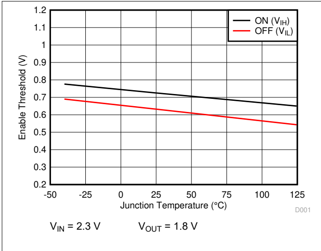
Figure 6-1. V_{EN} Threshold vs Temperature
