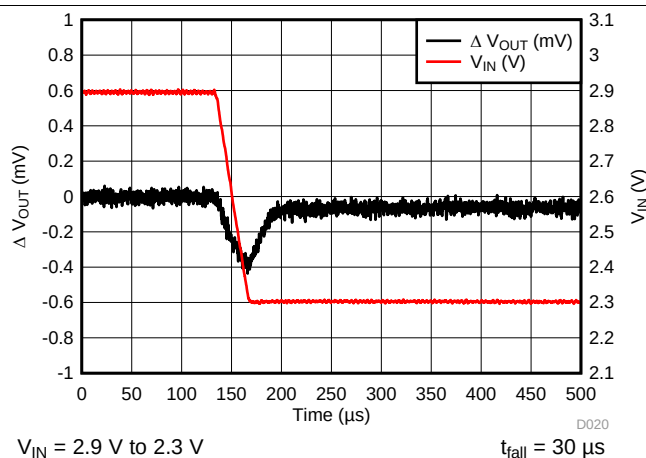
Figure 27. LP5912-0.9 Line Transient
