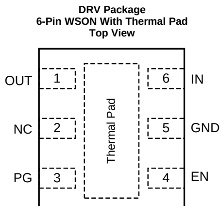
Pin Functions
