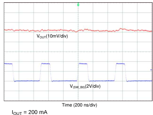
Figure 81. Output Voltage Ripple, Forced-PWM Mode (4-Phase Output)
