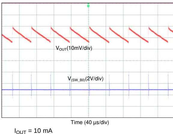
Figure 80. Output Voltage Ripple, PFM Mode (1-Phase Output)
