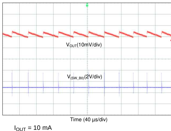
Figure 78. Output Voltage Ripple, PFM Mode (3-Phase Output)
