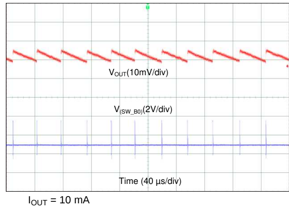
Figure 79. Output Voltage Ripple, PFM Mode (2-Phase Output)
