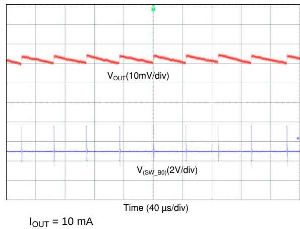
Figure 77. Output Voltage Ripple, PFM Mode (4-Phase Output)
