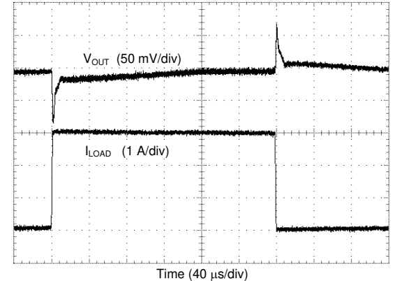
Figure 39. Transient Load Step Response, AUTO Mode
