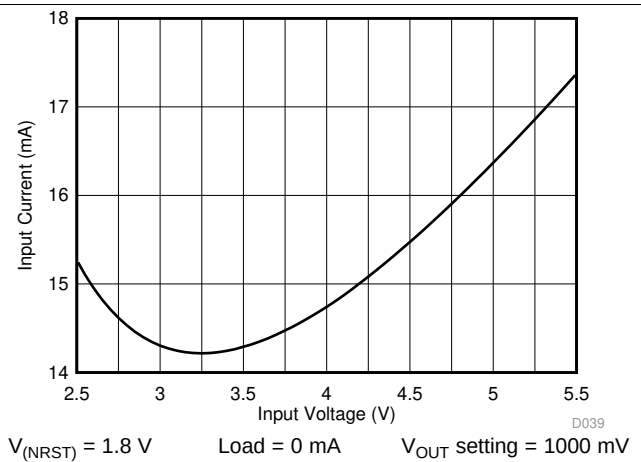
Figure 5. PWM Mode Current Consumption vs Input Voltage — One Output Enabled
