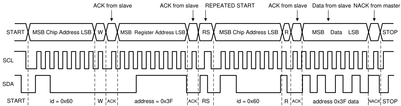
Figure 8-19. Read Cycle (r = read; SDA = 1), id = Device Address = 60Hex for LP87702-Q1
