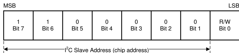
Figure 8-20. Device Address
