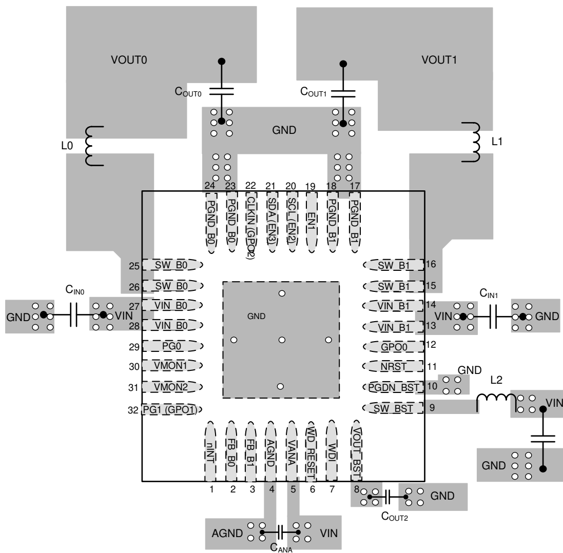
Figure 11-1. LP87702-Q1 Board Layout Example
