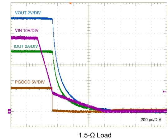
Figure 9-20. Shutdown By Input UVLO, 8-A Resistive Load
