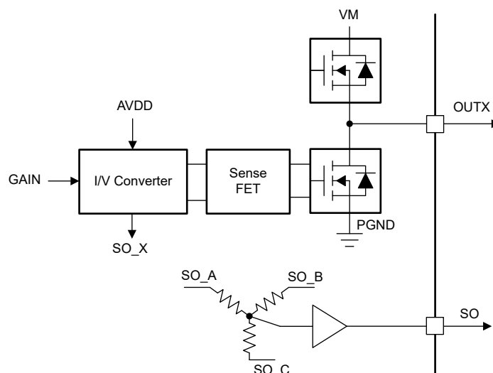
Figure 7-22. Integrated Current Sense Amplifier
