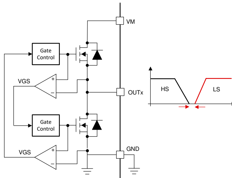
Figure 7-14. Cross Conduction Protection
