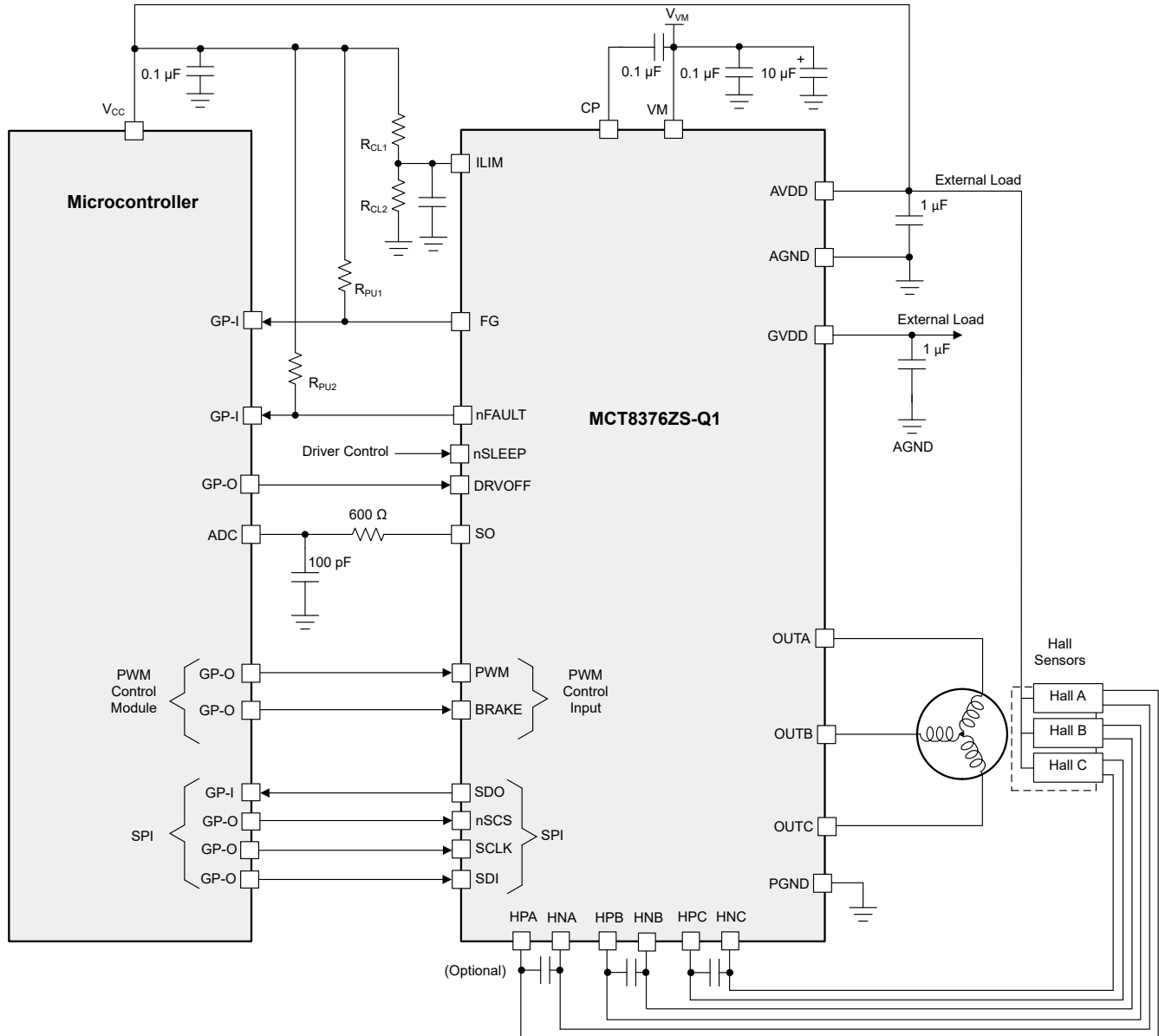
Figure 9-2. Primary Application Schematics for MCT8376ZS-Q1 (SPI variant)
