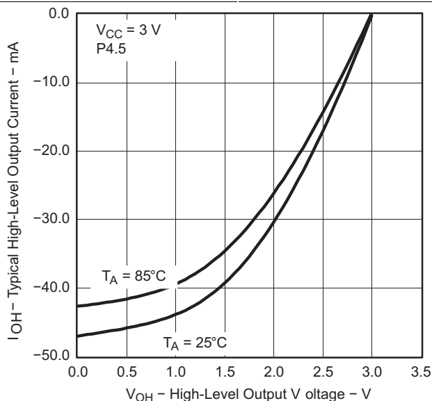
Figure 8. Typical High-Level Output Current vs High-Level Output Voltage
