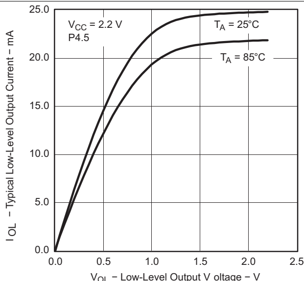
Figure 5. Typical Low-Level Output Current vs Low-Level Output Voltage
