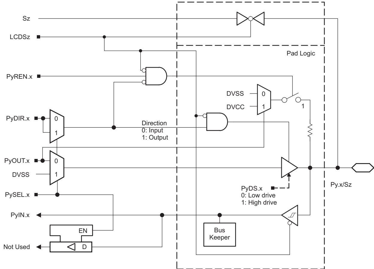
Figure 6-16. Port P4 (P4.0 to P4.7), Port P5 (P5.0 to P5.7), Port P6 (P6.0 to P6.7) Diagram (MSP430F67xxIPN Only)
