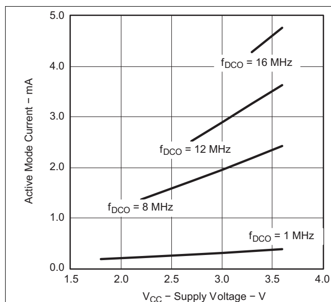
Figure 4. Active Mode Current vs V_{CC} , T_A = 25^\circ C
