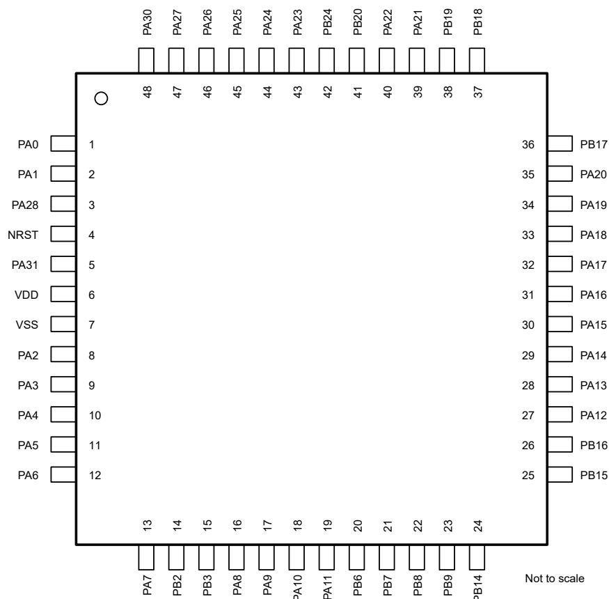
Figure 6-2. 48-pin PT 48-pin PT (LQFP) Package
