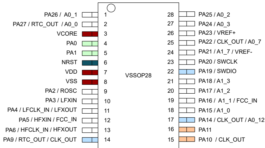
Figure 6-6. 28-Pin DGS28 (VSSOP) (Top View)
