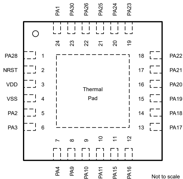
Figure 6-5. 24-Pin RGE (VQFN) (Top View)
