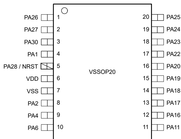
Figure 6-6. 20-Pin DGS20 (VSSOP) (Top View)
