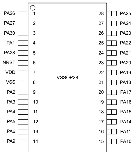
Figure 6-4. 28-Pin DGS28 (VSSOP) (Top View)
