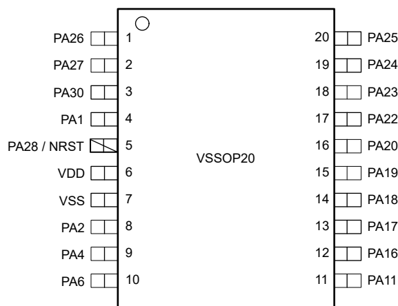
Figure 6-5. 20-Pin DGS20 (VSSOP) (Top View)
