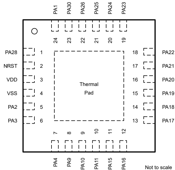
Figure 6-4. 24-Pin RGE (VQFN) (Top View)
