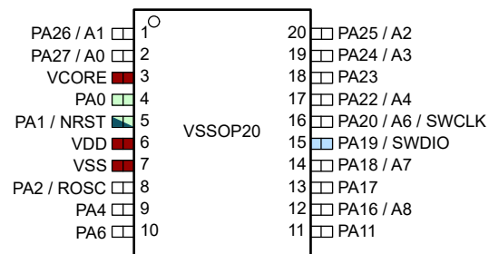
Figure 6-5. 20-Pin DGS20 (VSSOP) (Top View)
