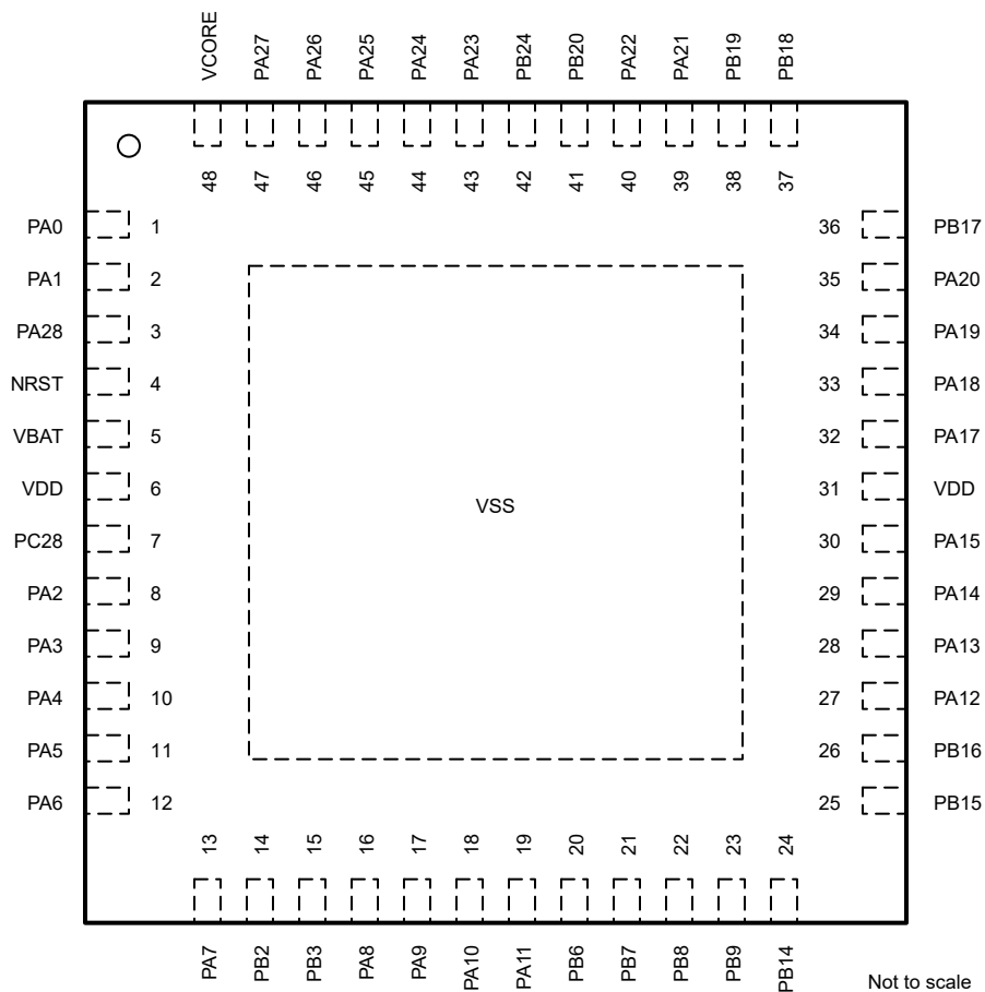
Figure 6-5. 48-pin RGZ (7mm x 7mm) (0.5mm pitch) (VQFN) Package Diagram (Top View)
