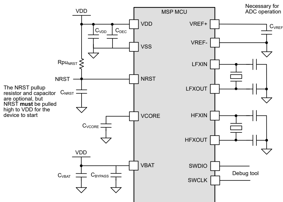
Figure 9-1. Basic Application Schematic
