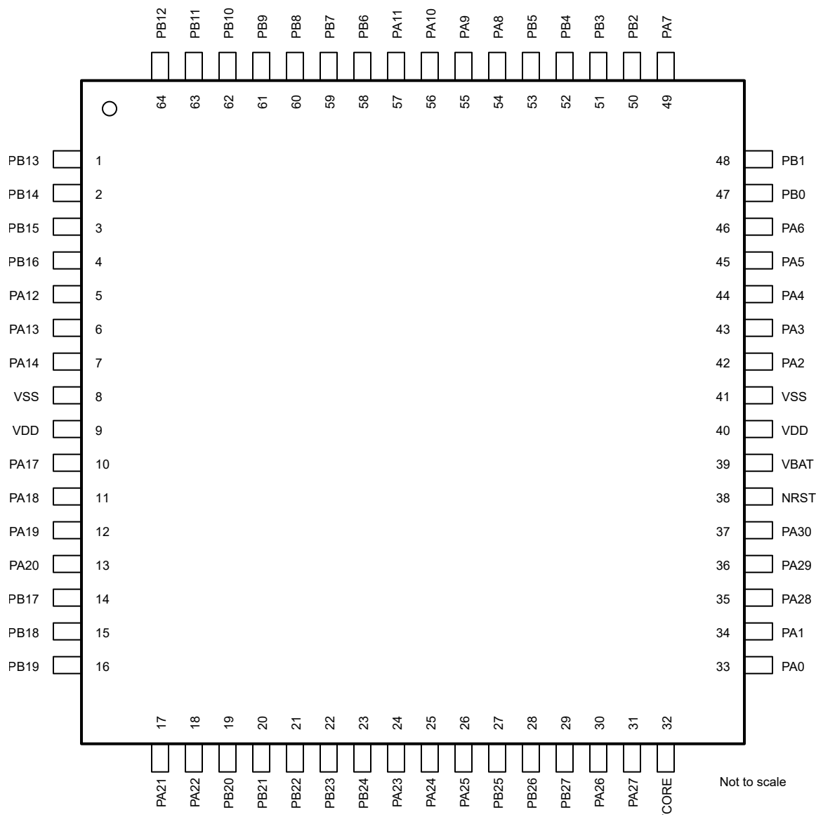
Figure 6-4. 64-pin PM (12mm x 12mm) (0.5mm pitch) (LQFP) Package Diagram (Top View)
