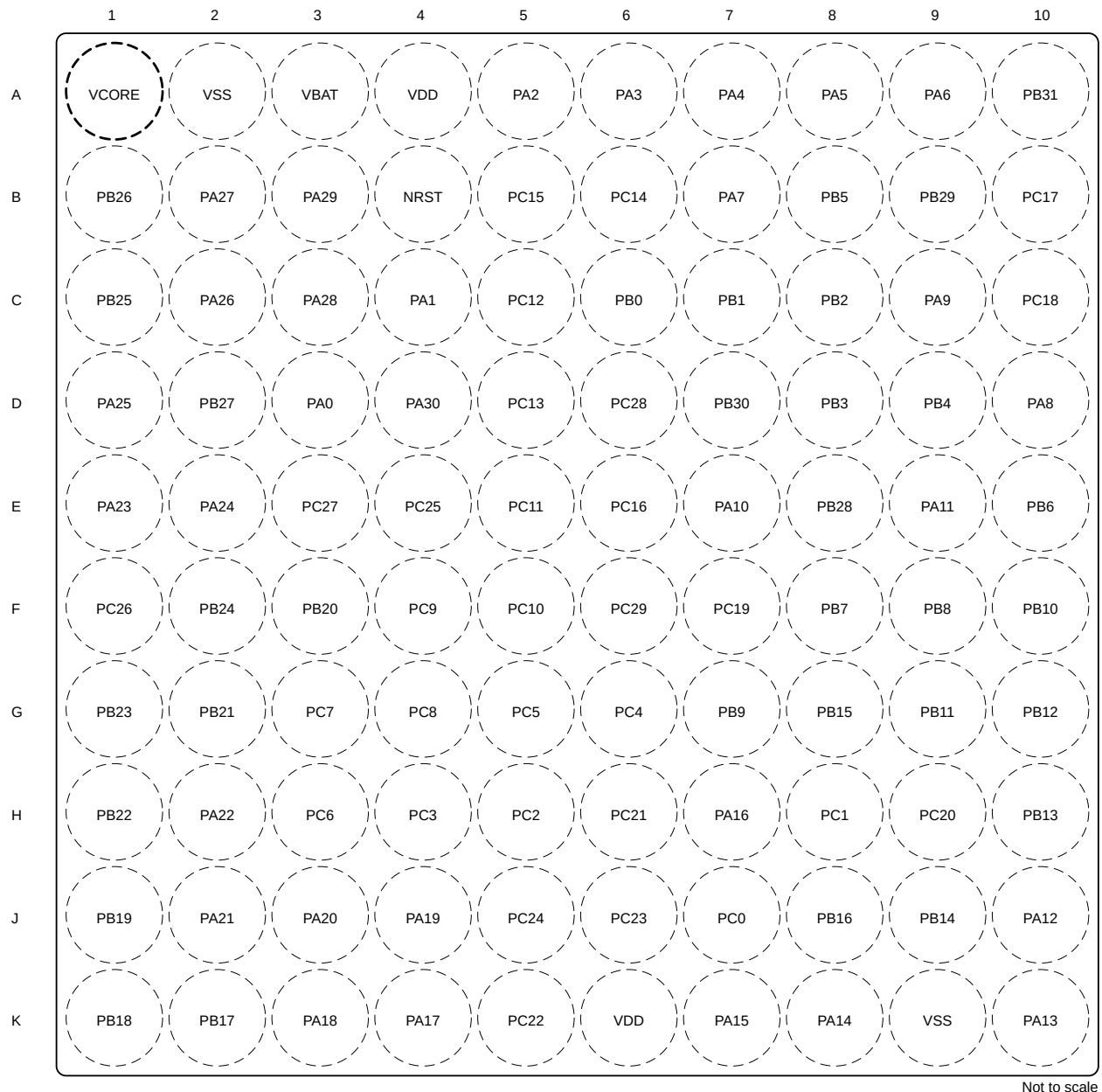
Figure 6-1. 100-pin ZAW (9mm x 9mm) (0.8mm pitch) (NFBGA) Package Diagram (Top View)
