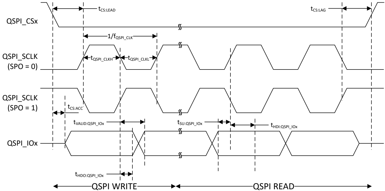
Figure 7-6. QSPI Timing Diagram - Controller Mode
