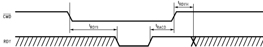
FIGURE 3-7. Ready Feedback Timing Diagram
