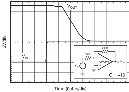
Figure 6-23. Positive Overload Recovery
