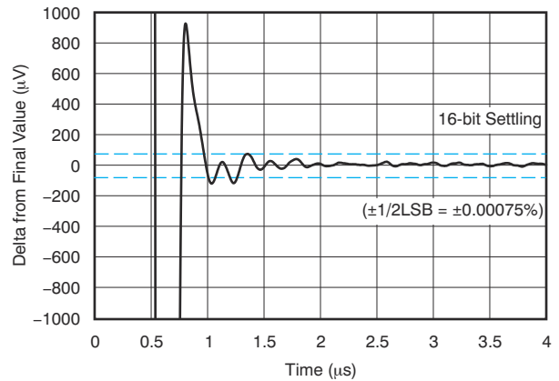
Figure 6-24. Negative Overload Recovery
