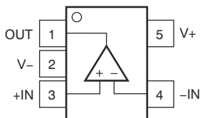
Figure 5-2. OPA140: DBV Package, 5-Pin SOT-23 (Top View)
