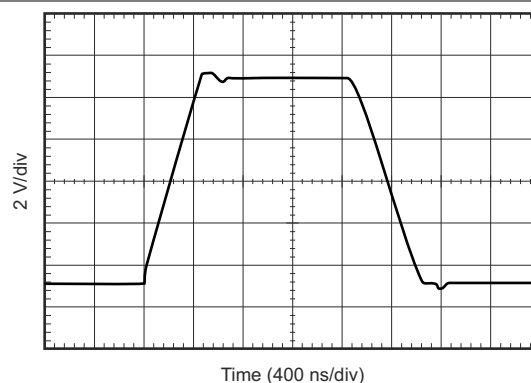
Figure 6-30. Large-Signal Step Response
