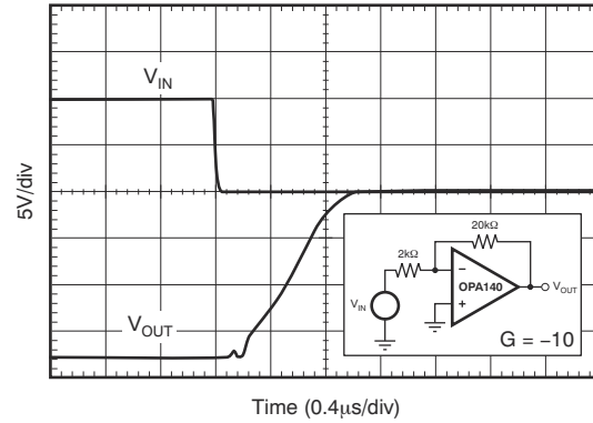
Figure 6-24. Negative Overload Recovery
