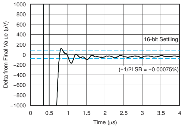
Figure 6-23. Positive Overload Recovery
