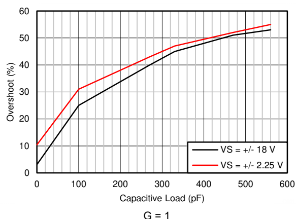
Figure 6-26. Percent Overshoot vs Capacitive Load
