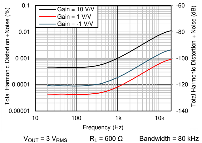
Figure 6-8. THD+N Ratio vs Frequency
