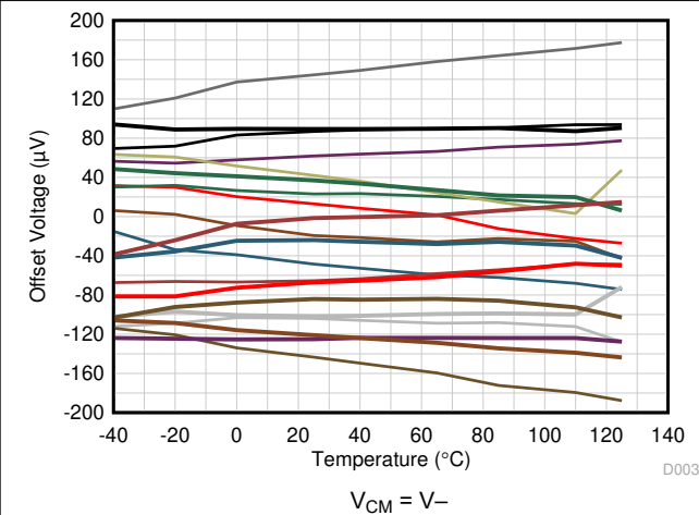
Figure 7-41. Offset Voltage vs Temperature (PMOS Input Pair)
