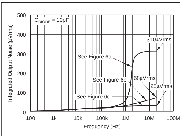
Figure 9. Integrated Output Noise for Circuits in Figure 6
