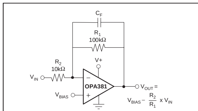
Figure 14. Inverting Gain
