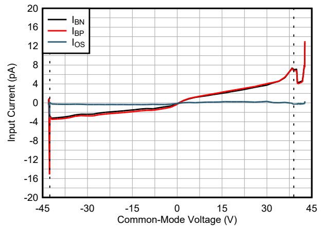
Figure 5-10. Input Bias vs Common-Mode Voltage
