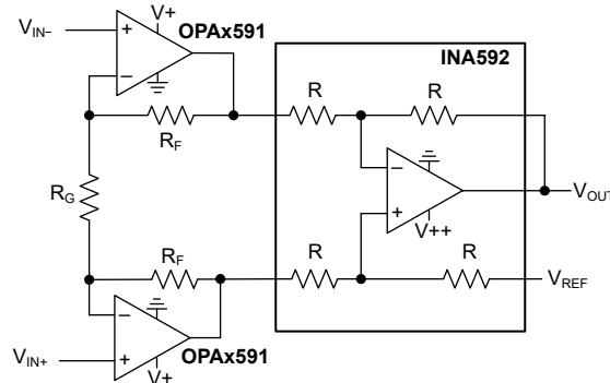
Figure 7-3. OPA591 Buffer for INA132
