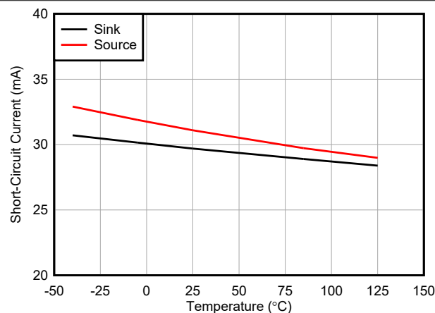
Figure 5-37. Short-Circuit Current vs Temperature
