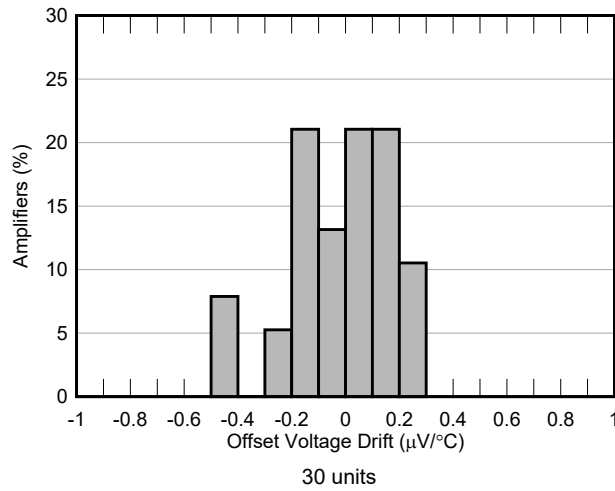
Figure 5-7. Offset Voltage Drift Distribution
