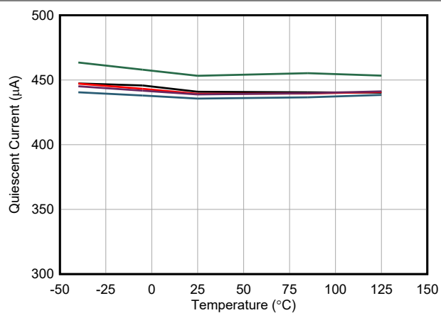
Figure 5-39. Quiescent Current vs Temperature
