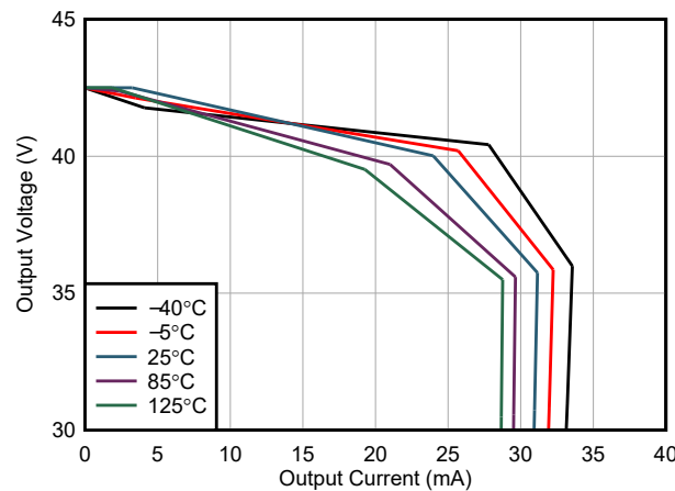
Figure 5-23. Output Voltage Swing vs Output Sourcing Current
