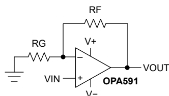
Figure 7-12. Schematic Representation of Noninverting Configuration
