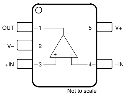
Figure 4-1. OPA591 DBV Package, 5-Pin SOT-23 (Top View)
