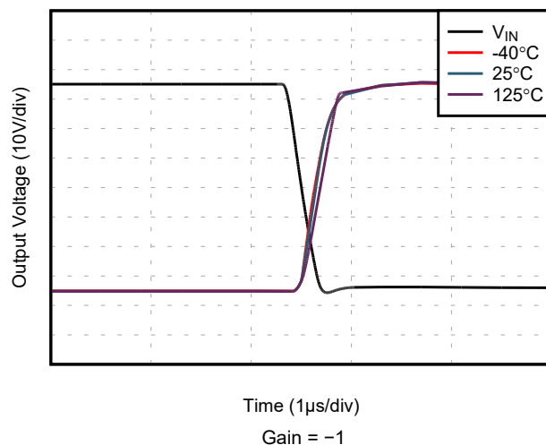
Figure 5-35. Large-Signal Step Response (Rising)
