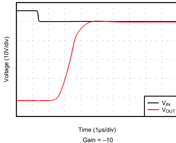
Figure 5-27. Negative Overload Recovery
