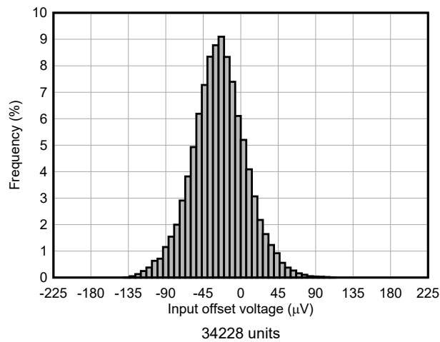
Figure 5-1. Offset Voltage Production Distribution at 25^\circ\text{C}
