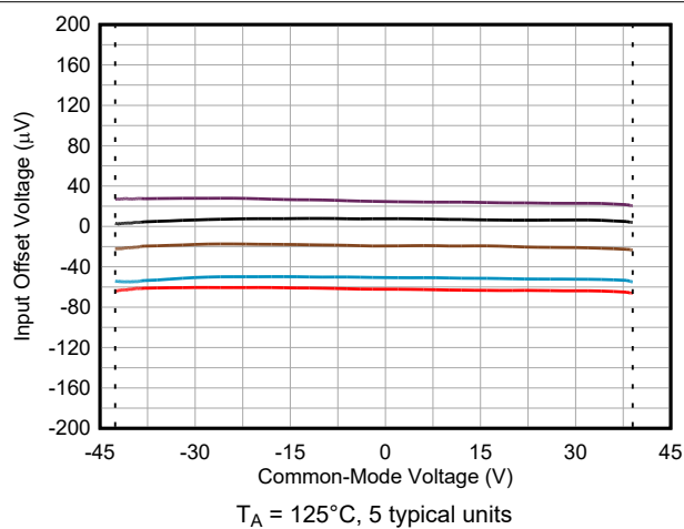
Figure 5-5. Input Offset Voltage vs Common-Mode Voltage
