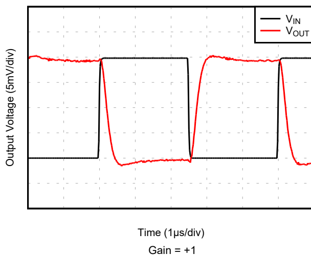
Figure 5-32. Small-Signal Step Response
