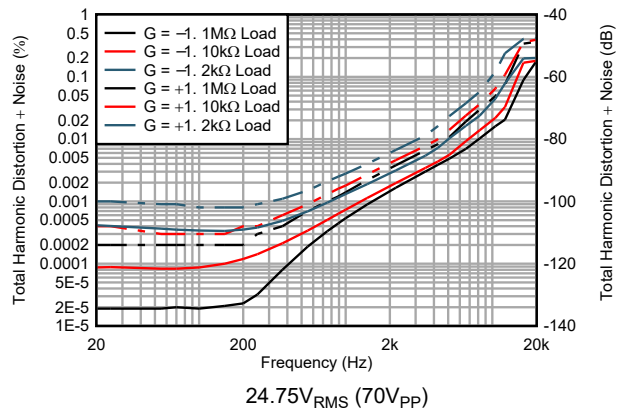
Figure 5-22. Total Harmonic Distortion + Noise Ratio vs Frequency
