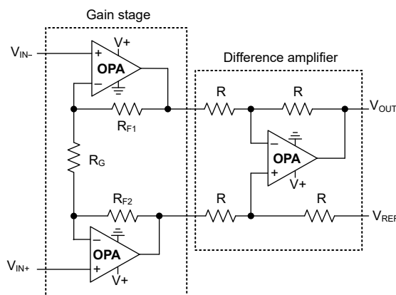
Figure 7-2. Instrumentation Amplifier
