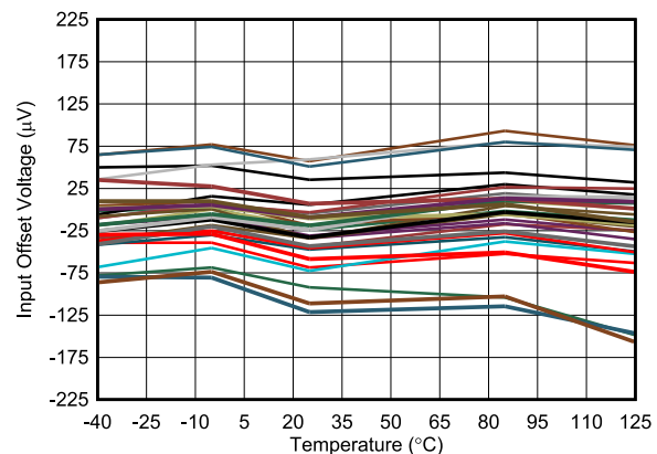
Figure 6-2. Input Offset Voltage Versus Temperature
