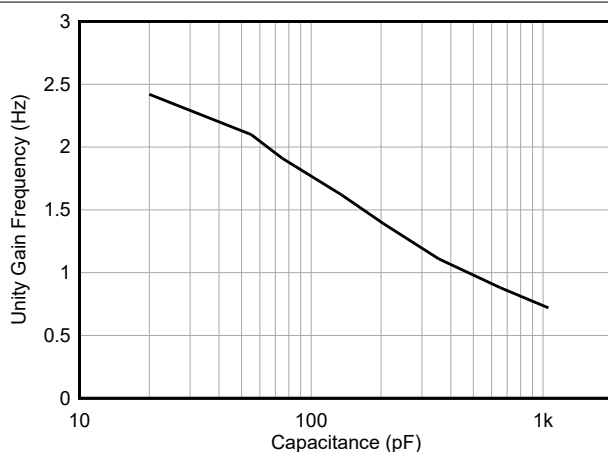
Figure 5-17. Unity-Gain Bandwidth vs Capacitive Load
