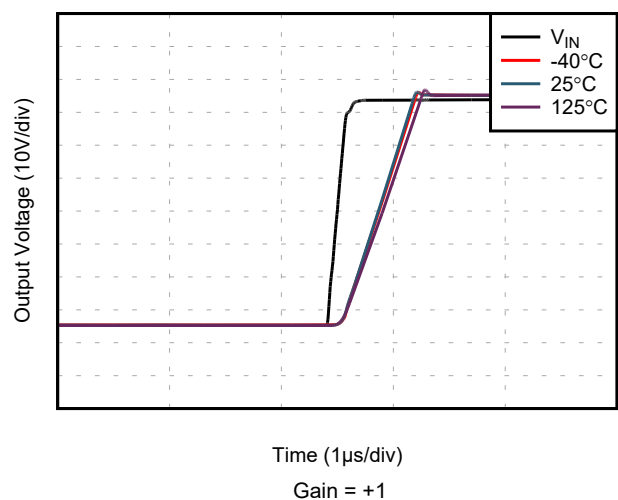
Figure 5-34. Large-Signal Step Response (Rising)
