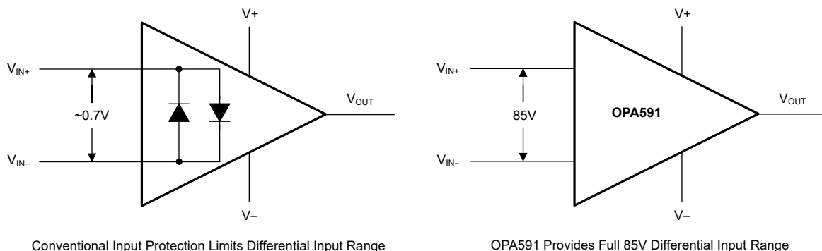
Figure 6-3. OPA591 Input Protection Does Not Limit Differential Input Capability
