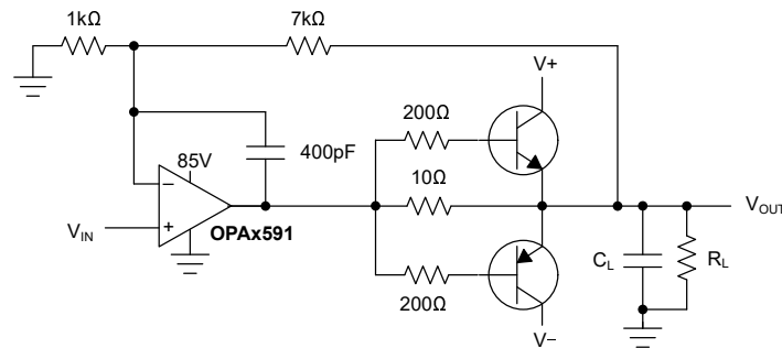
Figure 7-8. Current Booster Circuit
