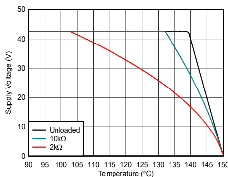
Figure 7-9. OPA591 (SOT23-5) Thermal Safe Operating Area
