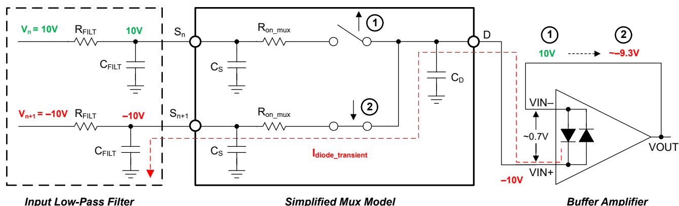
Figure 6-4. Back-to-Back Diodes Create Settling Issues
