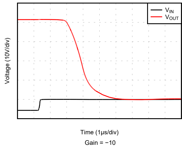
Figure 5-26. Positive Overload Recovery
