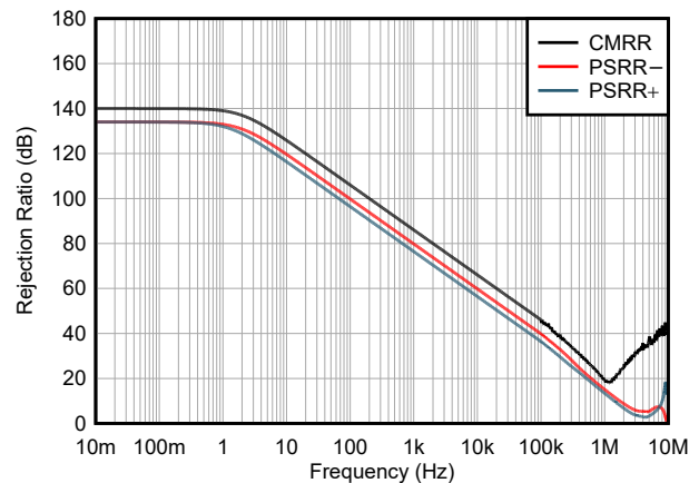
Figure 5-12. Power-Supply and Common-Mode Rejection Ratio vs Frequency
