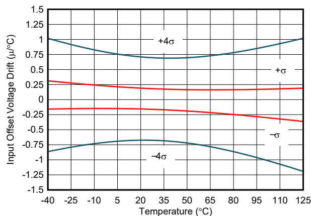
Figure 6-1. Input Offset Voltage Drift Versus Temperature
