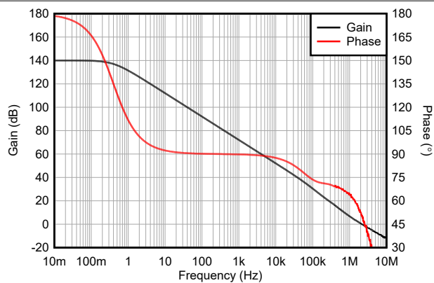
Figure 5-15. Open-Loop Gain and Phase vs Frequency
