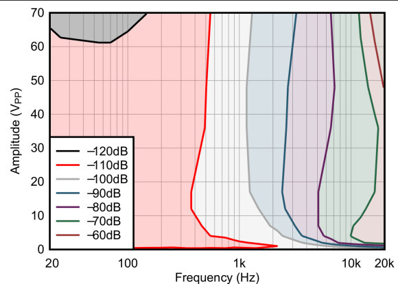
Figure 6-6. Full-Power Bandwidth Improved
