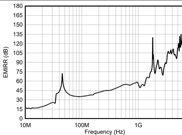
Figure 5-40. Electromagnetic Interference Rejection
