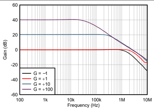
Figure 5-16. Closed-Loop Gain vs Frequency
