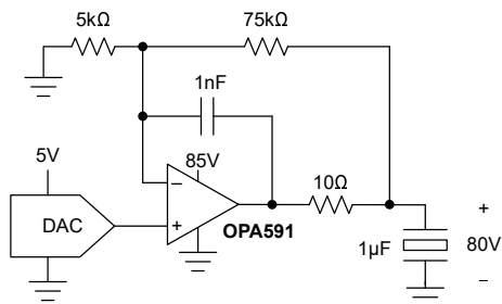
Figure 7-7. 80V Single-Supply Piezoelectric Driver
