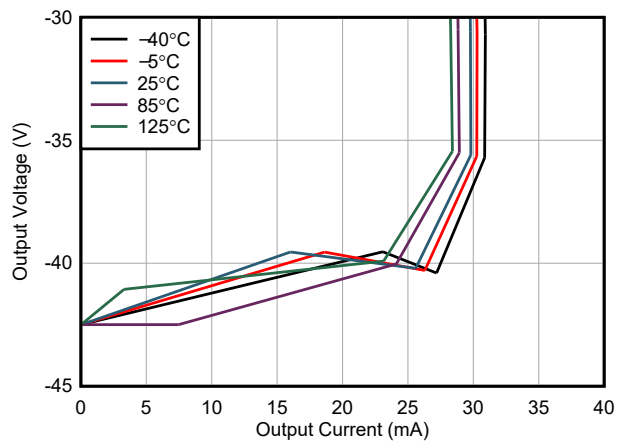
Figure 5-24. Output Voltage Swing vs Output Sinking Current
