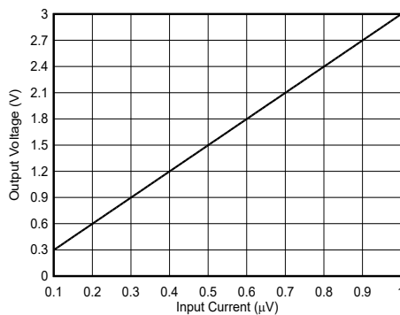
Figure 7-4. Output Voltage
