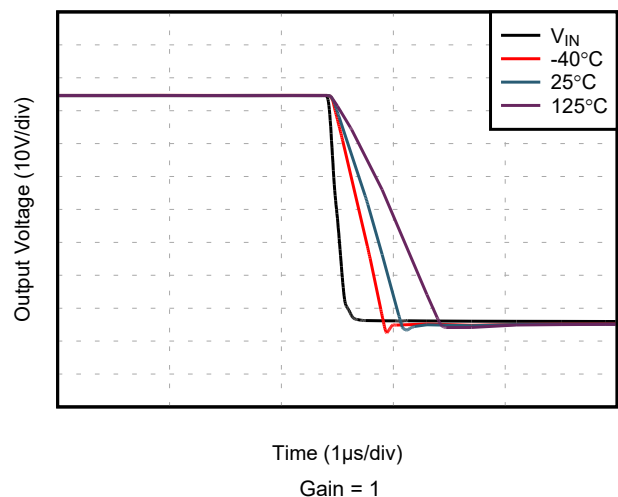
Figure 5-36. Large-Signal Step Response (Falling)
