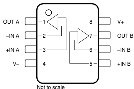
Figure 4-2. OPA2591 D Package, 8-Pin SOIC and DGK Package, 8-Pin VSSOP (Top View)
