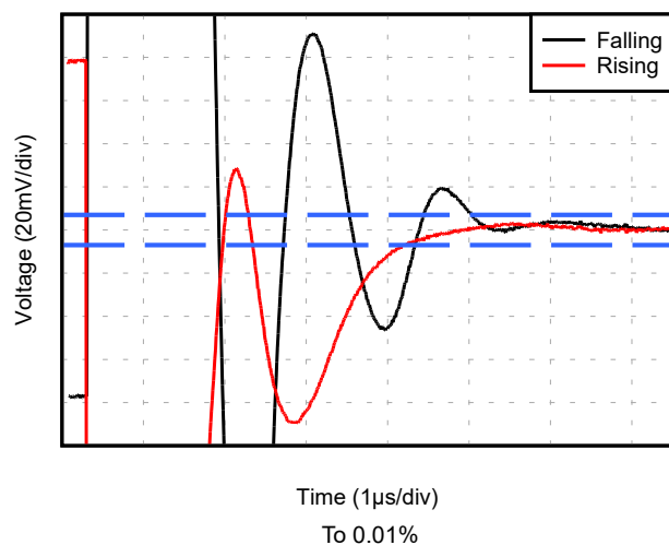
Figure 5-31. Settling Time
