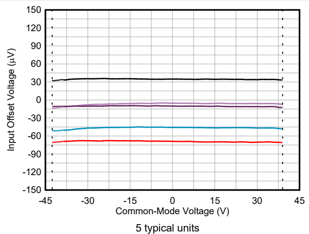
Figure 5-4. Input Offset Voltage vs Common-Mode Voltage
