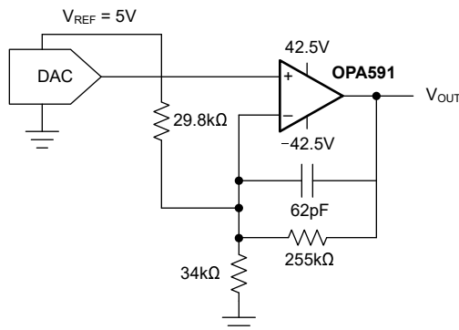
Figure 7-6. DAC Output Gain and Buffer
