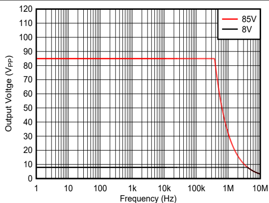
Figure 6-5. Full-Power Bandwidth
