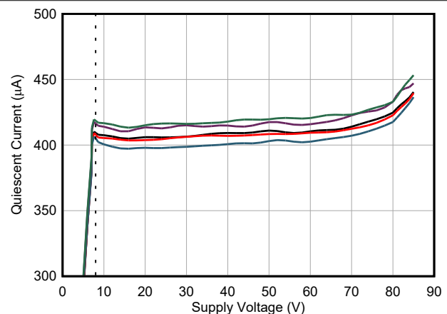
Figure 5-38. Quiescent Current vs Supply Voltage
