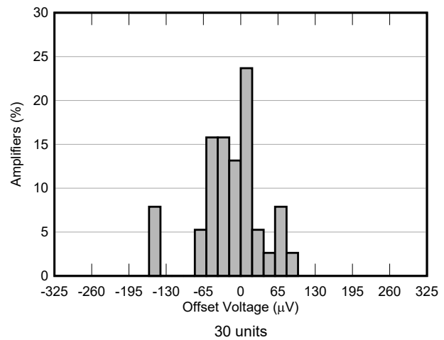
Figure 5-2. Offset Voltage Production Distribution at 125^\circ\text{C}
