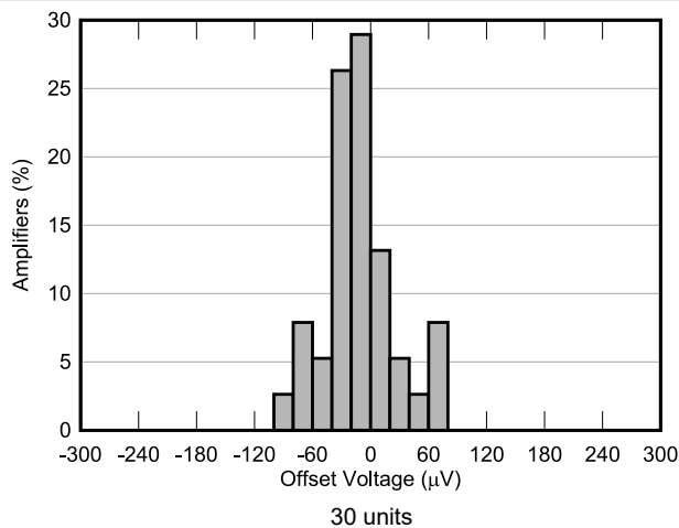
Figure 5-3. Offset Voltage Production Distribution at -40^\circ\text{C}
