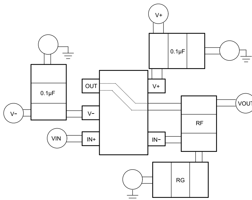
Figure 7-13. Board Layout for Noninverting Configuration of the SOT23-5 Package
