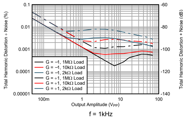
Figure 5-21. Total Harmonic Distortion + Noise Ratio vs Output Amplitude
