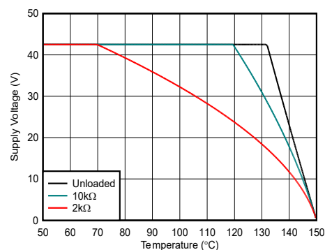
Figure 7-10. OPA2591 (VSSOP-8) Thermal Safe Operating Area
