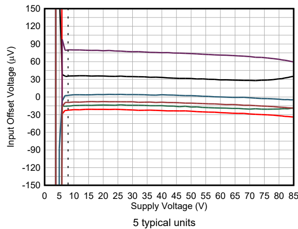
Figure 5-9. Offset Voltage vs Power Supply Voltage
