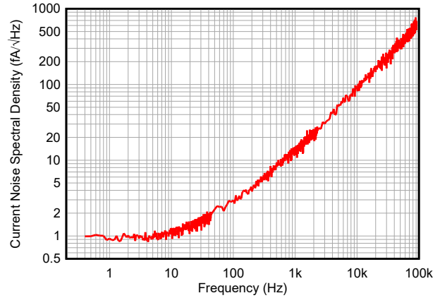
Figure 5-20. Current Noise Density vs Frequency
