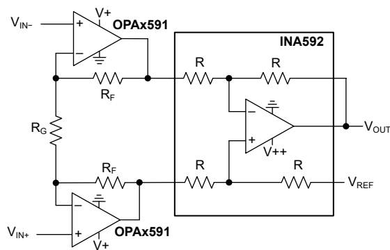
OPA591 Buffer With INA592
