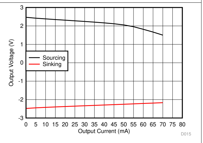
Figure 41. Output Voltage Range vs Output Current
