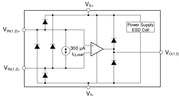
Figure 63. Internal ESD Protection
