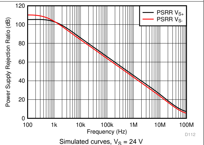
Figure 55. Power Supply Rejection Ratio vs Frequency
