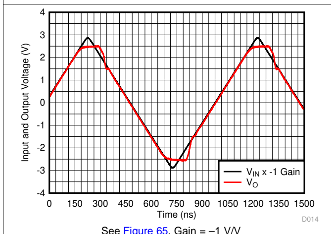
Figure 40. Output Overdrive Recovery
