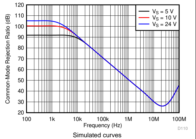
Figure 53. Common-Mode Rejection Ratio vs Frequency
