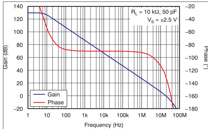
Figure 1. Open-Loop Gain and Phase vs Frequency
