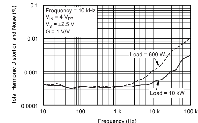
Figure 19. THD+N vs Frequency
