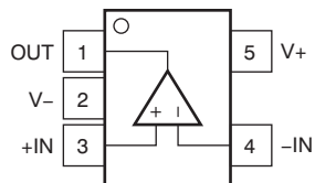
Pin Functions: OPA322-Q1
