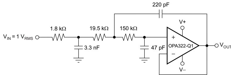
Figure 34. OPAx322-Q1 Configured as a Three-Pole, 20-kHz, Sallen-Key Filter
