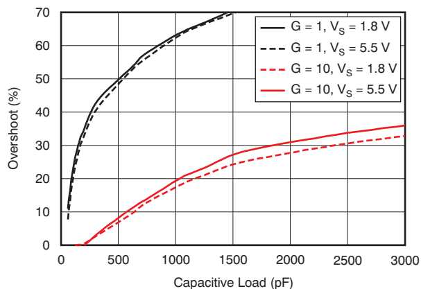
Figure 29. Small-Signal Overshoot vs Capacitive Load (100-mV pp Output Step)
