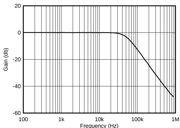
Figure 36. OPAx322-Q1 Second-Order, 50-kHz, Low-Pass Filter
