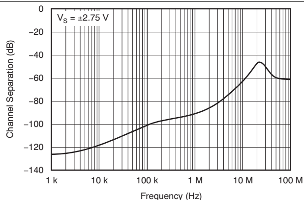
Figure 20. Channel Separation vs Frequency (Dual-Channel)
