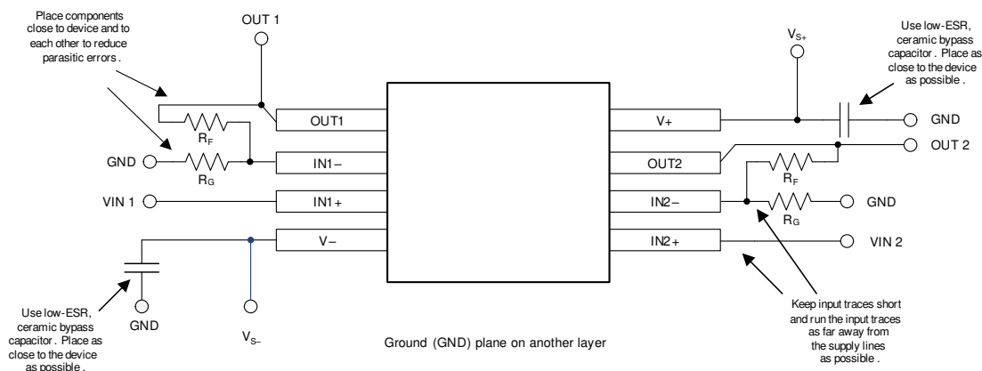
Figure 7-4. Layout Example
