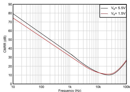
Figure 5-20. CMRR vs Frequency
