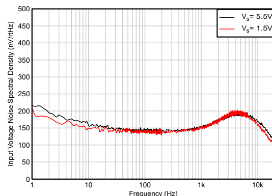
Figure 5-24. Input Voltage Noise Spectral Density
