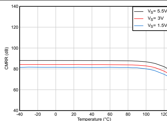
Figure 5-22. DC CMRR vs Temp ( (V_-) \geq V_{CM} \geq (V_+) - 0.7\text{V} )
