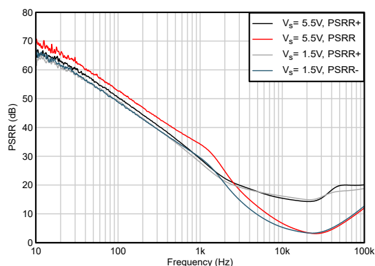
Figure 5-19. PSRR vs Frequency
