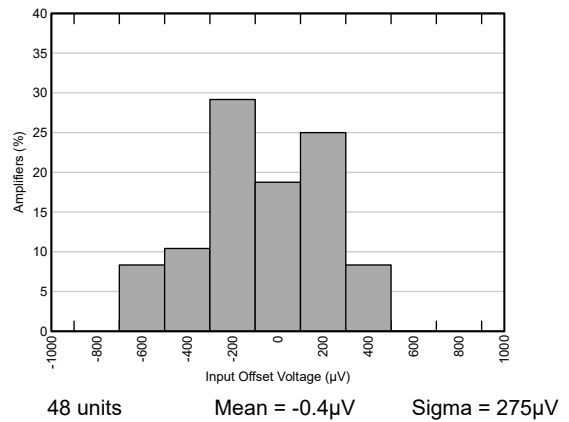
Figure 5-2. Offset Voltage Histogram ( V_S = 1.5\text{V} )
