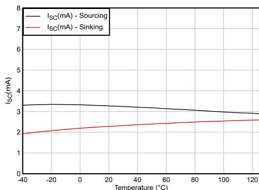
Figure 5-39. Short-Circuit Current vs Temperature ( V_S = 1.5\text{V} )
