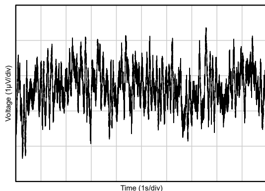
Figure 5-23. 0.1Hz to 10Hz Voltage Noise in Time Domain
