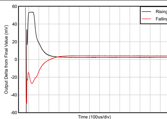
Figure 5-34. Large-Signal Step Response
