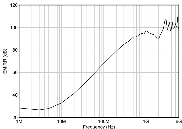
Figure 6-4. EMIRR Testing
