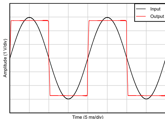
Figure 5-37. No Phase Reversal
