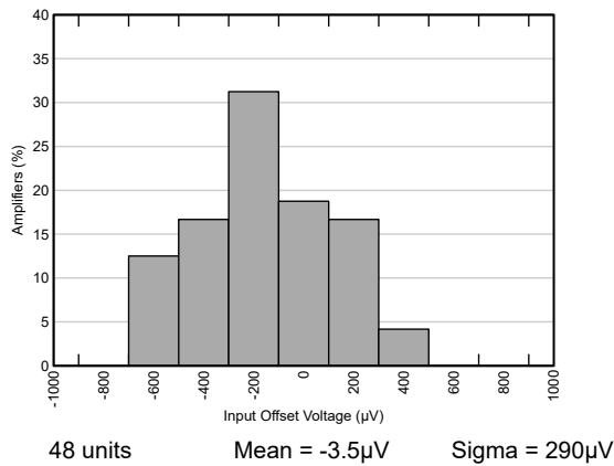
Figure 5-1. Offset Voltage Histogram
