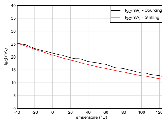
Figure 5-38. Short-Circuit Current vs Temperature ( V_S = 5.5\text{V} )
