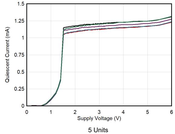
Figure 6-26. Quiescent Current vs Supply Voltage
