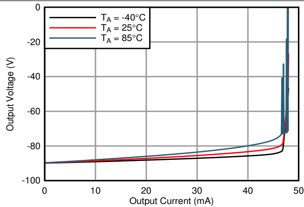
Figure 31. Negative Output Voltage vs Output Current
