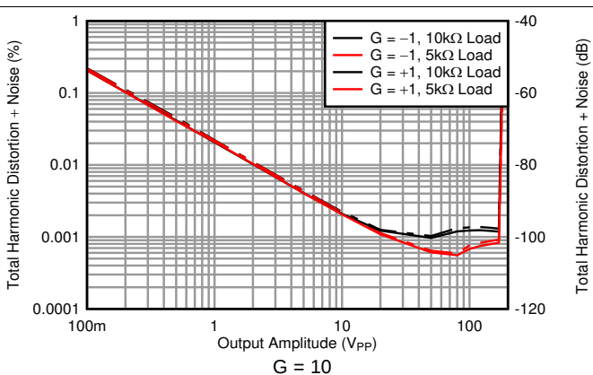
Figure 48. THD+N Ratio vs Output Amplitude
