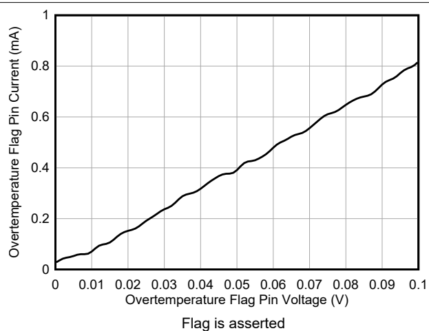
Figure 6-74. Overtemperature Flag Pin Current vs Overtemperature Flag Pin Voltage
