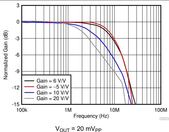
Figure 7-4. Small-Signal Frequency Response vs Gain
