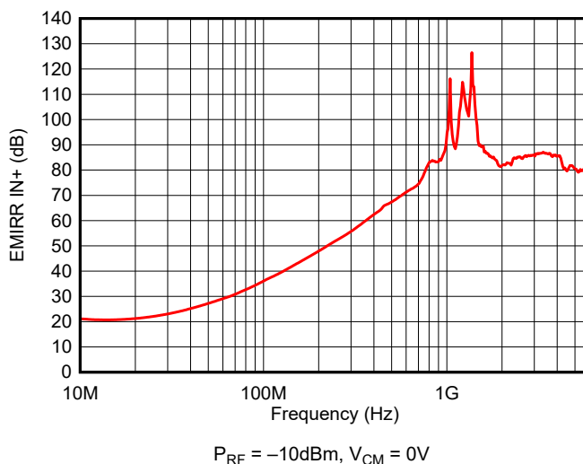
Figure 6-2. EMIRR Testing
