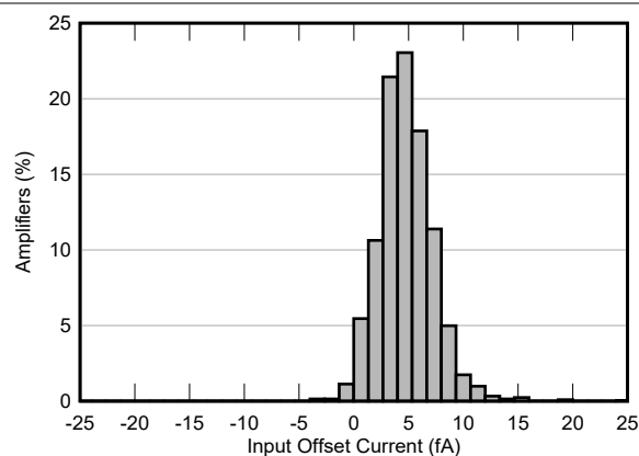
Figure 5-8. Input Bias Offset Current Production Distribution
