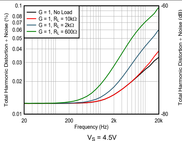
Figure 5-42. THD+N vs Frequency
