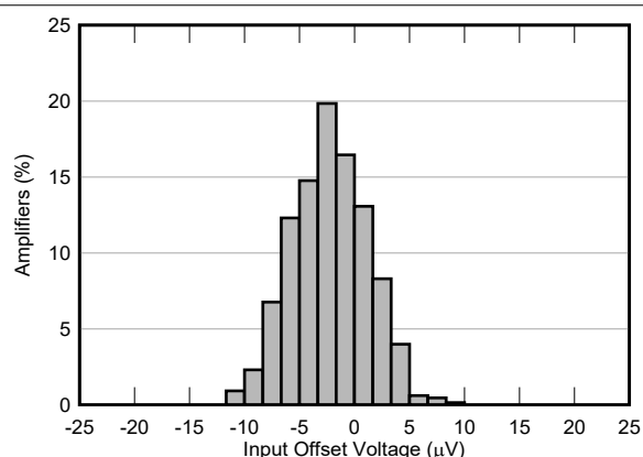
Figure 5-9. Offset Voltage Production Distribution
