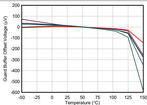
Figure 5-74. Guard Buffer Offset Voltage vs Temperature
