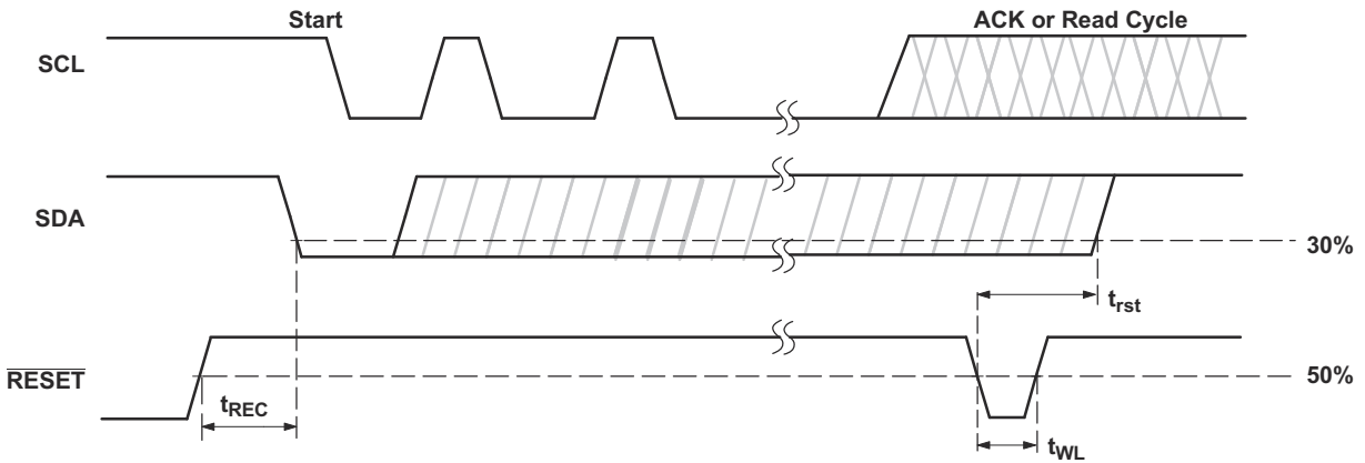
Figure 7-2. Reset Timing
