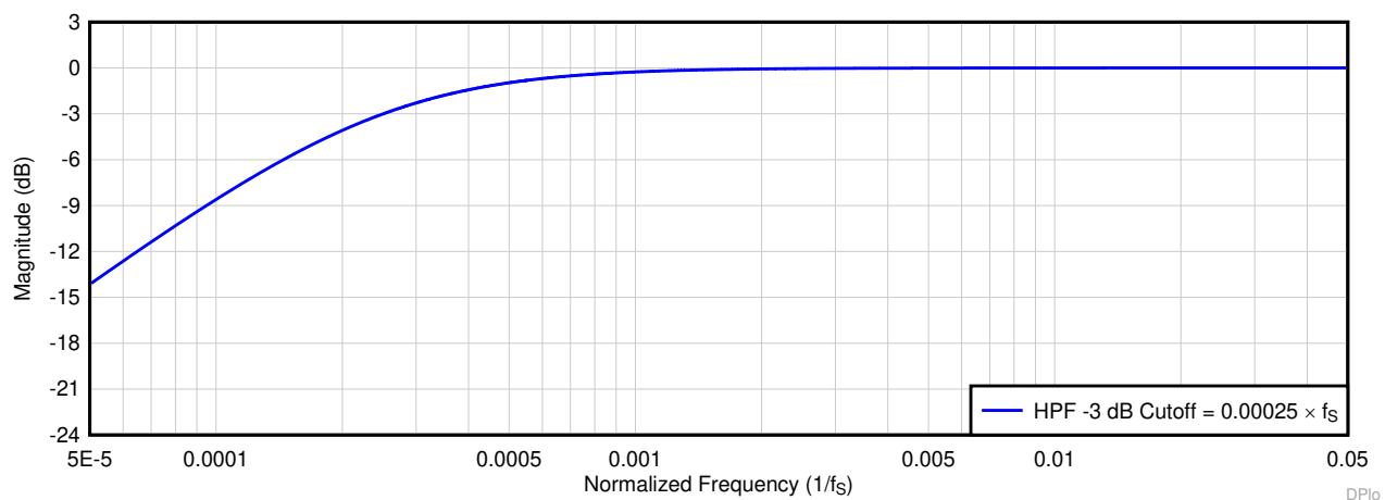
Figure 8-6. HPF Filter Frequency Response Plot
