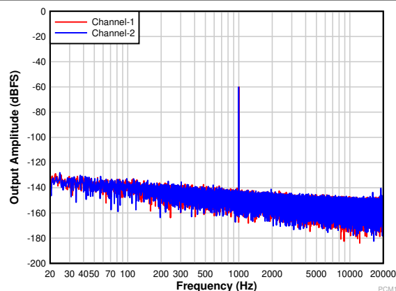
Figure 9-6. PCM1821: FFT With a –60-dBr Input
