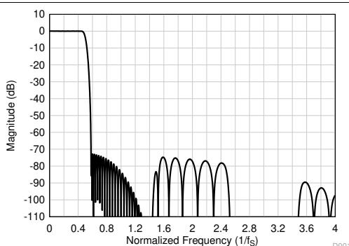
Figure 8-7. Linear Phase Decimation Filter Magnitude Response
