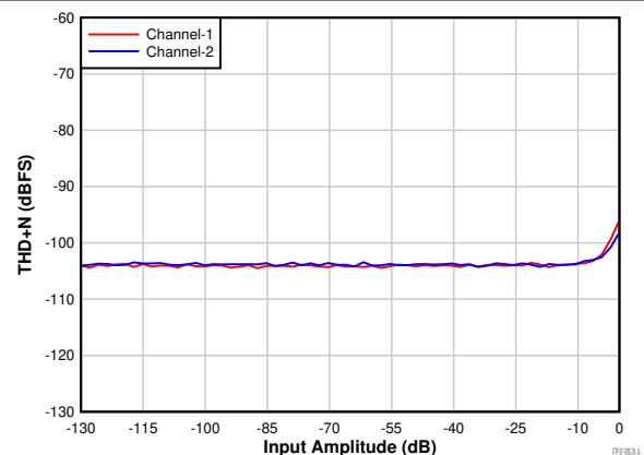
Figure 9-7. PCM1821: THD+N vs Input Amplitude
