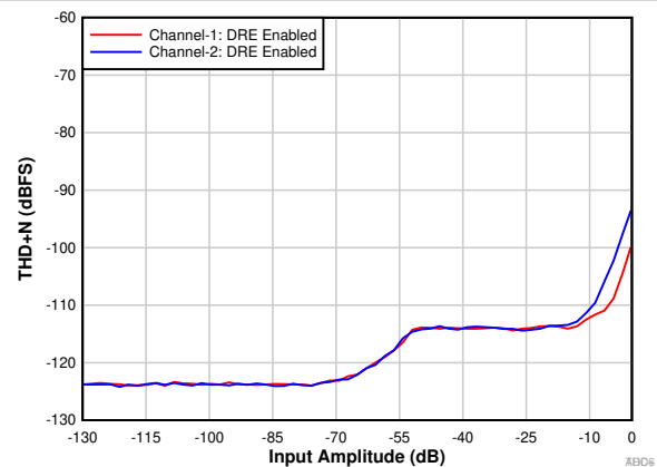
Figure 9-3. PCM1820: THD+N vs Input Amplitude With DRE Enabled
