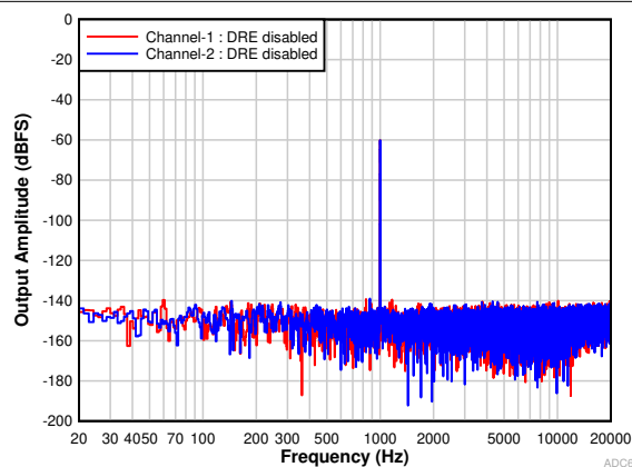
Figure 9-4. PCM1820: FFT With a –60-dBr Input With DRE Disabled
