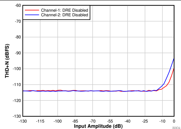
Figure 9-5. PCM1820: THD+N vs Input Amplitude With DRE Disabled
