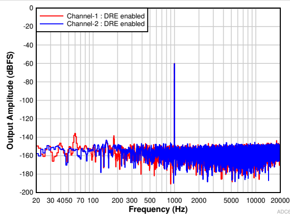
Figure 9-2. PCM1820: FFT With a –60-dBr Input With DRE Enabled
