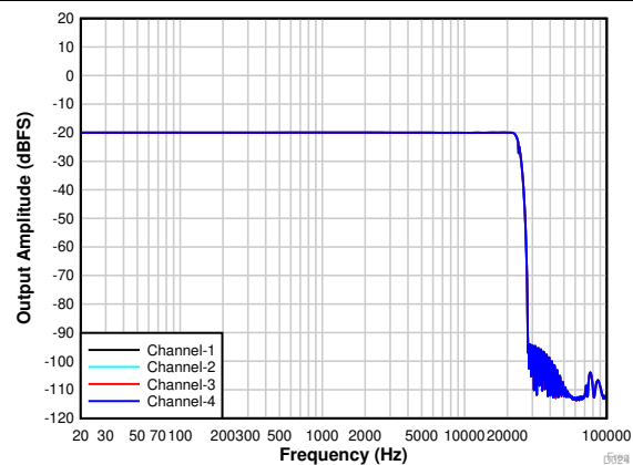
Figure 7-31. PDM Input Frequency Response With a -20\text{-dBr} Input
