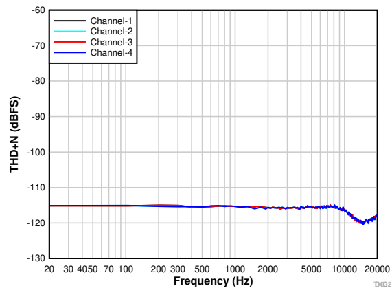
Figure 7-29. PDM Input THD+N vs Input Frequency With a -20\text{-dBr} Input
