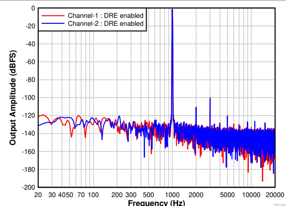
Figure 7-26. Differential FFT With a -1-dBr Input With DRE Enabled
