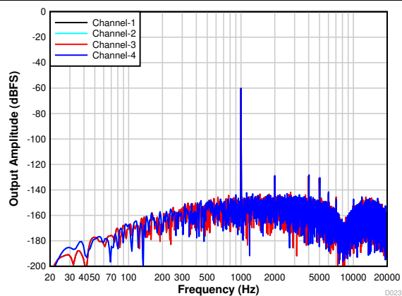
Figure 7-30. PDM Input FFT With a -60\text{-dBr} Input
