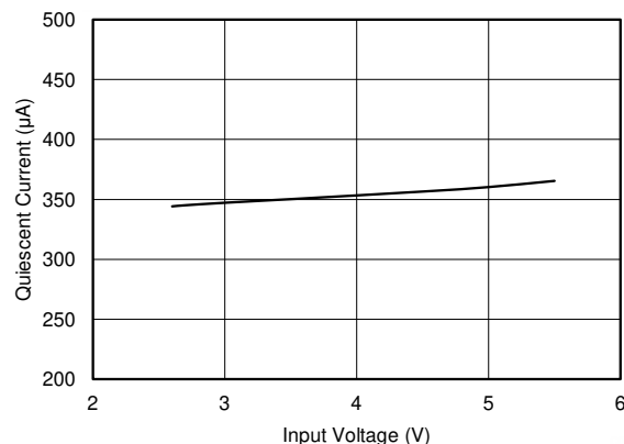
Figure 6-28. Quiescent Current vs Input Voltage
