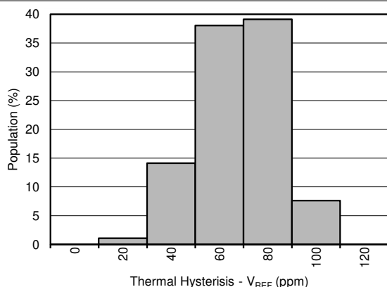
Figure 7-4. Thermal Hysteresis Distribution (V REF )
