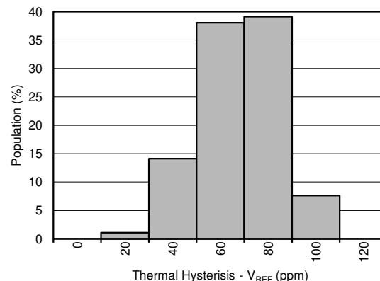
Figure 6-34. Thermal Hysteresis Distribution ( V_{REF} )
