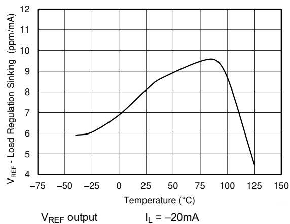
Figure 6-12. Load Regulation Sinking vs Temperature ( V_{REF} )
