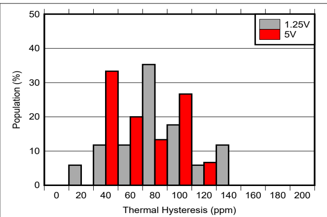
Figure 6-26. Thermal Hysteresis Histogram -40°C to 85°C Cycle 1
