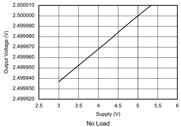
Figure 6-39. Output Voltage vs Supply Voltage
