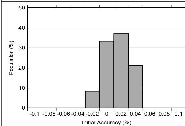
Figure 6-5. Initial Accuracy
