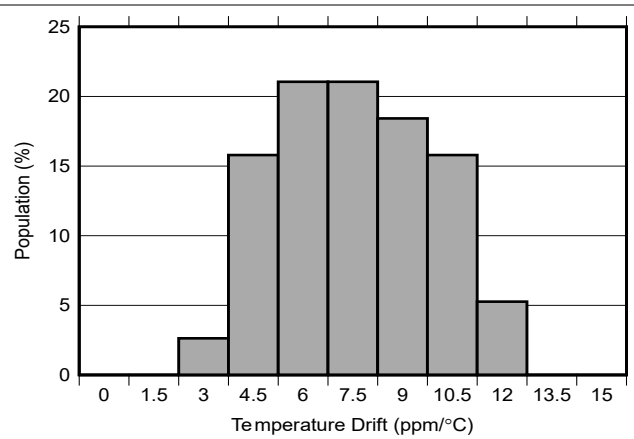
Figure 6-2. Temperature Drift Histogram -40°C to +85°C
