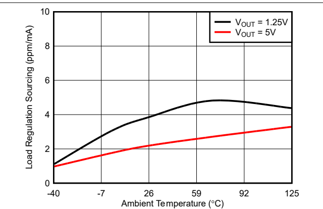
Figure 6-6. Load Regulation Sourcing vs Temperature
