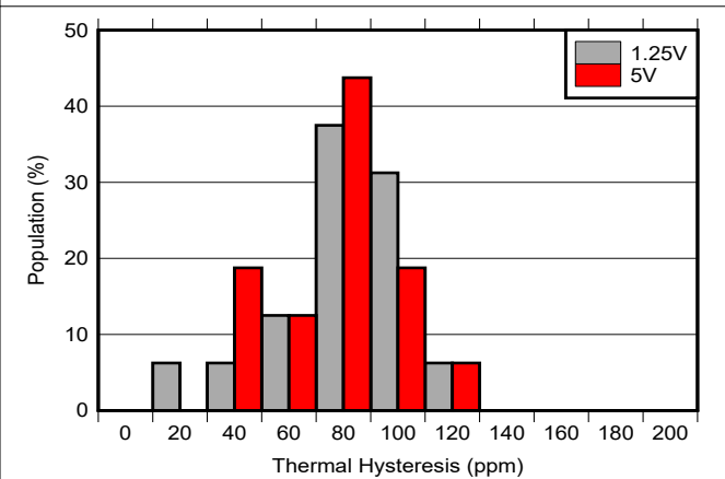
Figure 6-28. Thermal Hysteresis Histogram 0°C to 70°C Cycle 1
