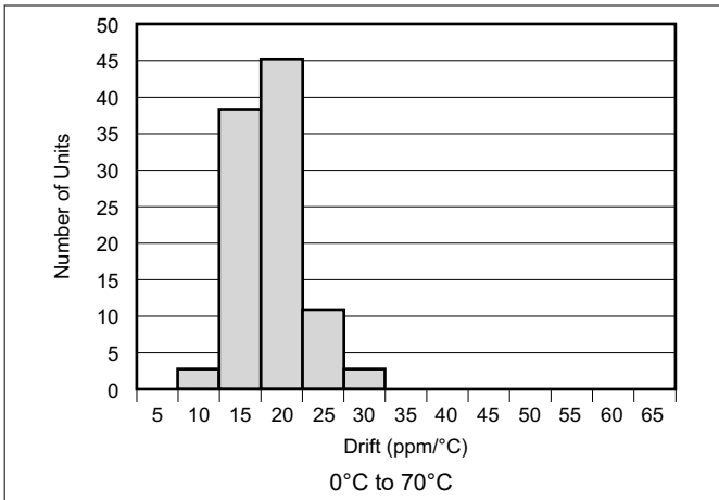
Figure 6-30. Temperature Drift
