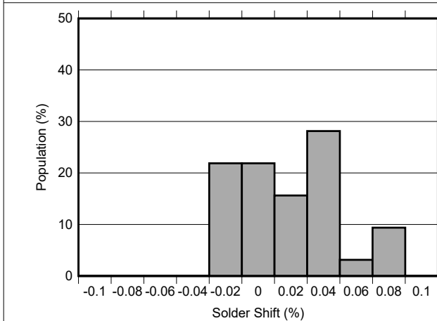
Figure 6-15. Solder Shift Histogram
