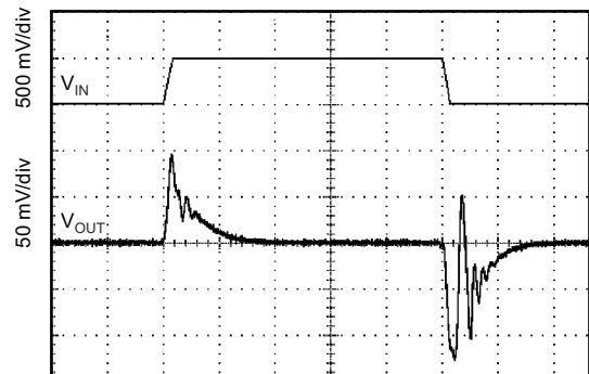
Figure 6-42. Step Response
