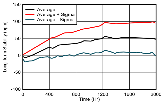
Figure 6-23. Long-Term Stability: 0 to 2000 Hours
