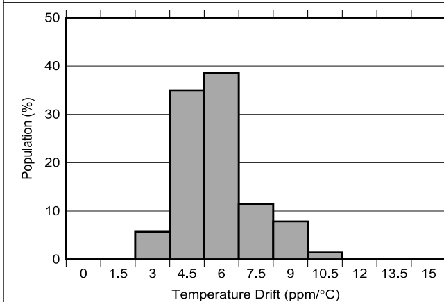
Figure 6-3. Temperature Drift Histogram 0°C to +70°C
