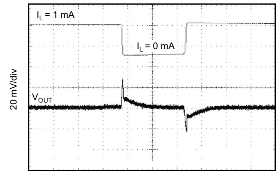
Figure 6-43. Step Response
