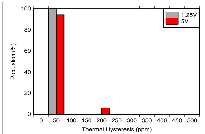
Figure 6-25. Thermal Hysteresis Histogram -40°C to 125°C Cycle 2
