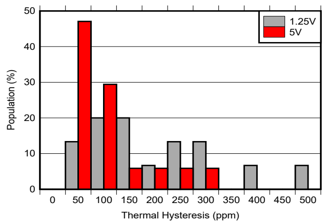
Figure 6-24. Thermal Hysteresis Histogram -40°C to 125°C Cycle 1
