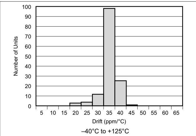
Figure 6-31. Temperature Drift
