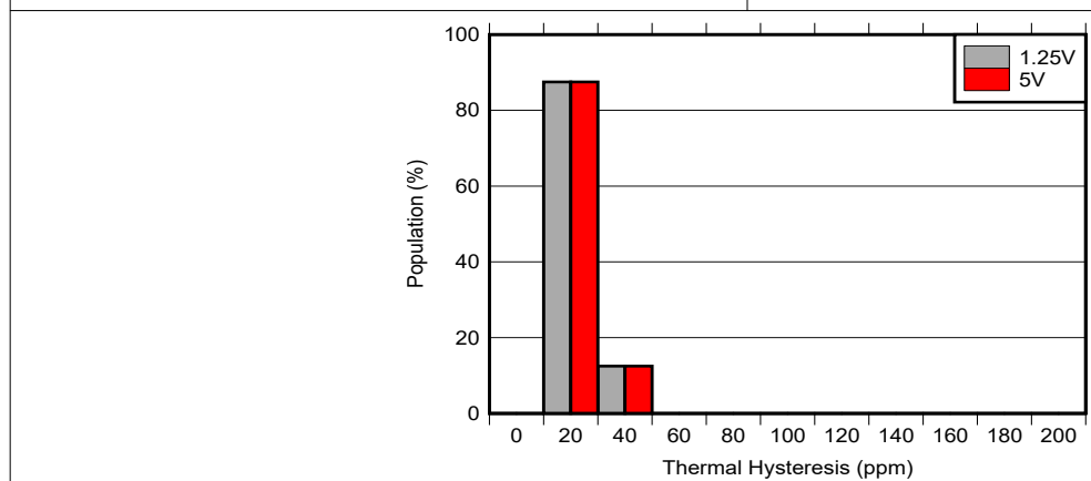
Figure 6-29. Thermal Hysteresis Histogram 0°C to 70°C Cycle 2
