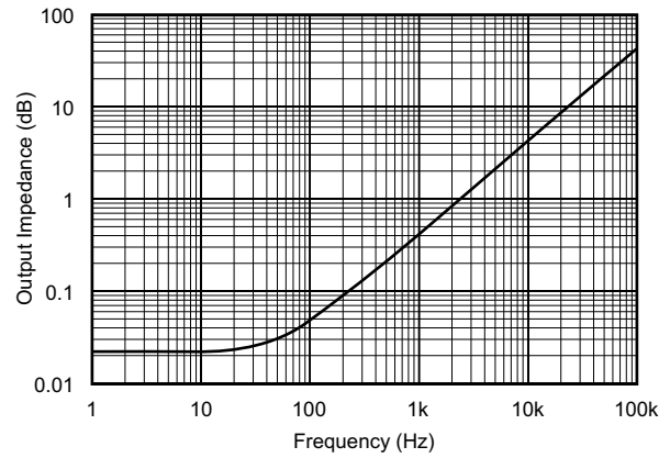
Figure 6-37. Output Impedance vs Frequency
