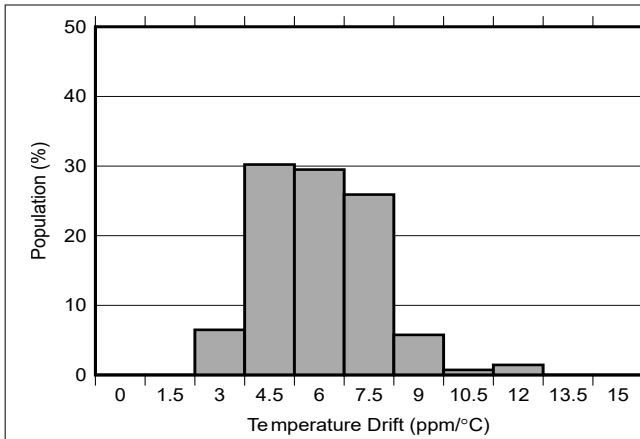
Figure 6-1. Temperature Drift Histogram -40°C to +125°C
