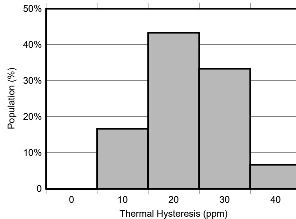
Figure 8-8. REF7012QFKHR Thermal Hysteresis Distribution (-40°C to 125°C)
