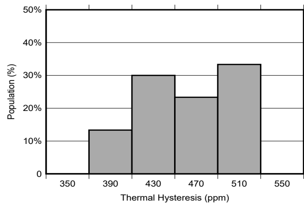
Figure 8-7. REF7012QDGKR Thermal Hysteresis Distribution (-40°C to 125°C)
