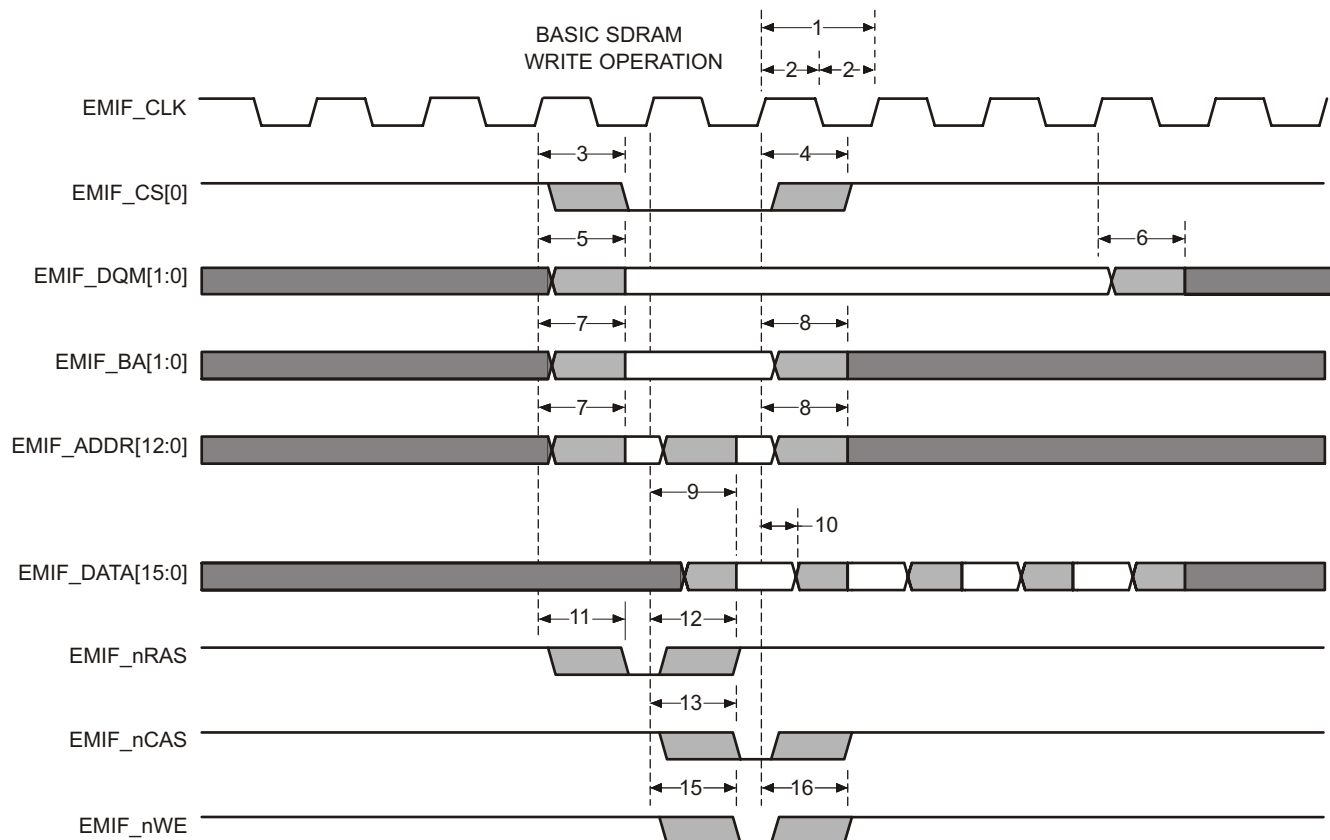
Figure 6-17. Basic SDRAM Write Operation
