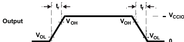
Figure 5-3. CMOS-Level Outputs
