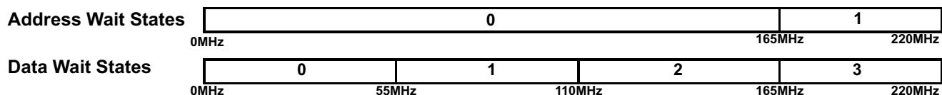
Figure 5-1. Wait States Scheme
