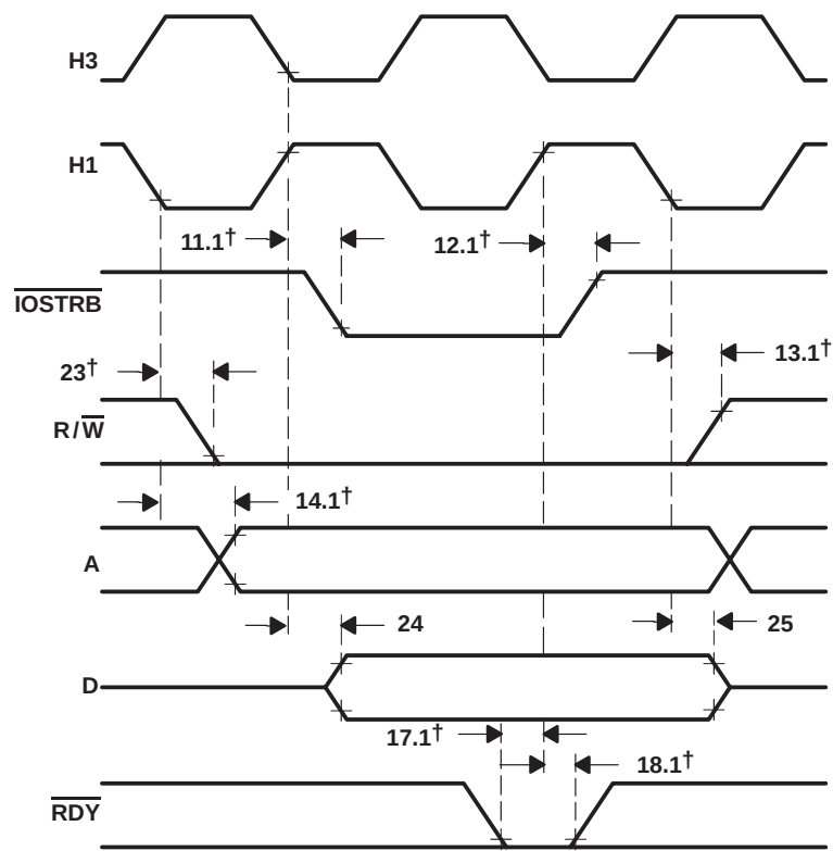
Figure 19. Memory-Write-Cycle Timing Using \overline{\text{IOSTRB}}
