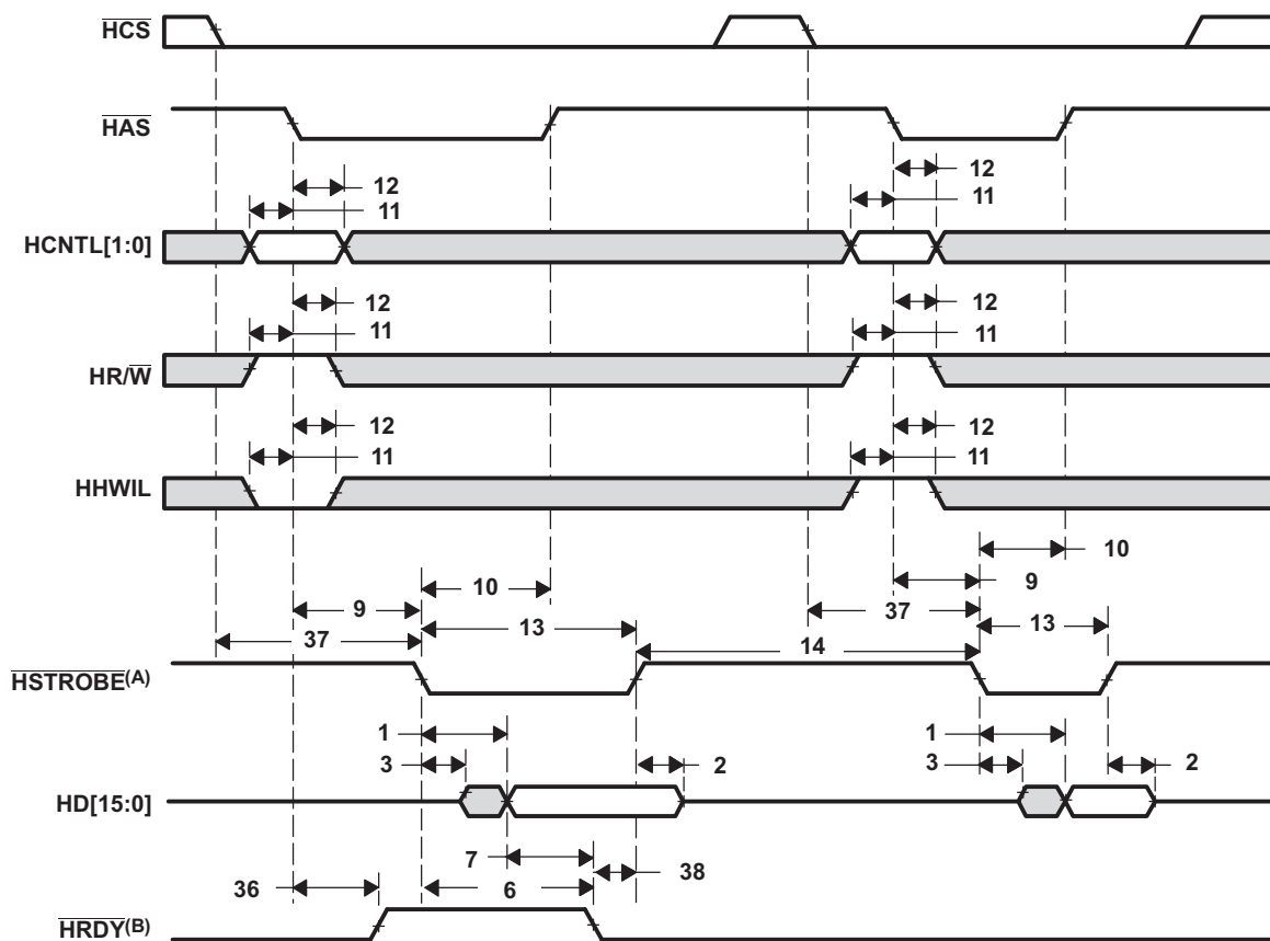
Figure 4-44. HPI16 Read Timing ( \overline{\text{HAS}} Used)
