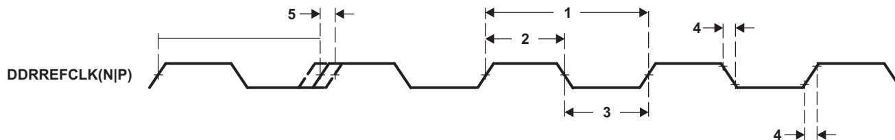
Figure 4-30. DDRREFCLK(N|P) Timing
