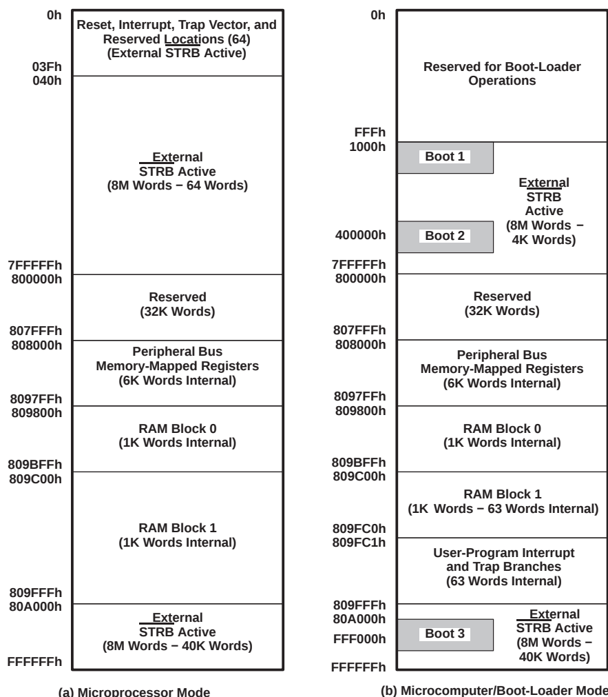
Figure 1. SM320C31-EP Memory Map
